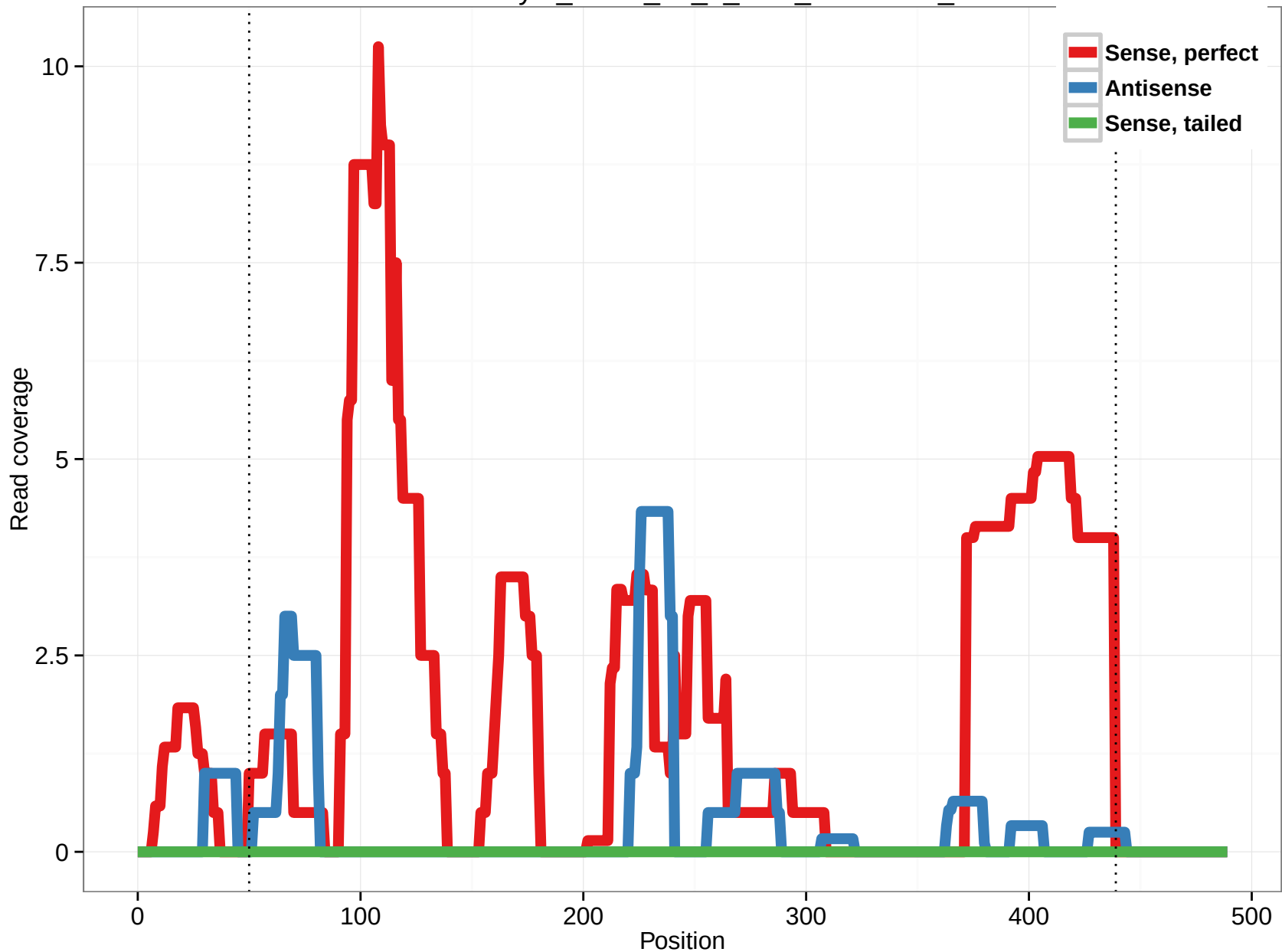
uc004amy.2_intron_11_0_chr9_86432043_r
