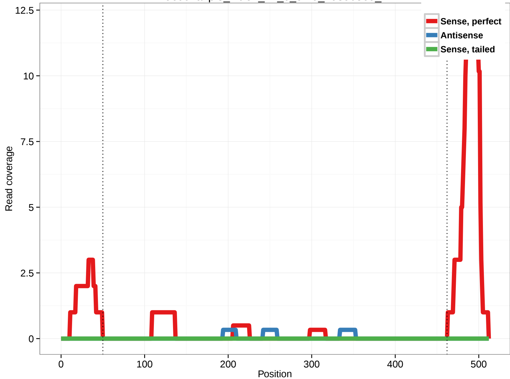
uc004akp.3_intron_24_0_chr9_79890569_f
