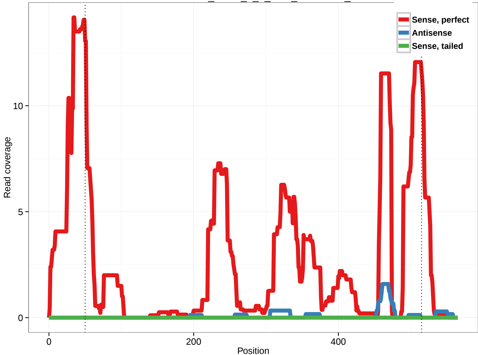
uc004ach.2_intron_0_0_chr9_42469104_f
