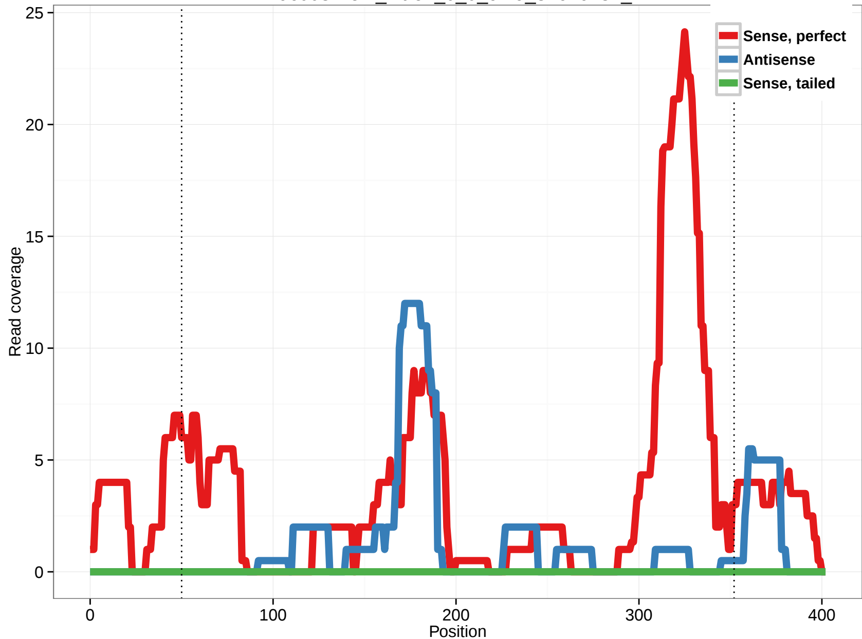
uc003zve.2_intron_0_0_chr9_34646784_f
