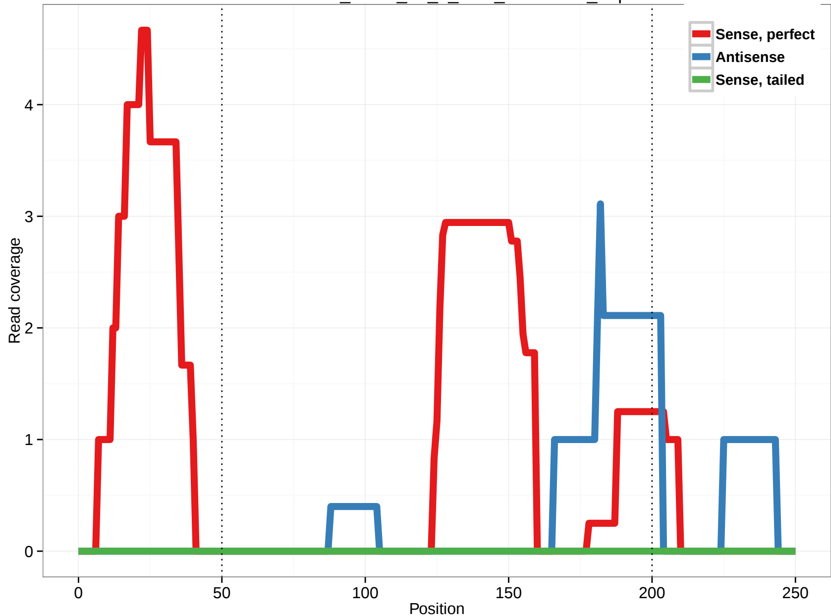
uc003znk.2_intron_14_0_chr9_19094394_r.5p
