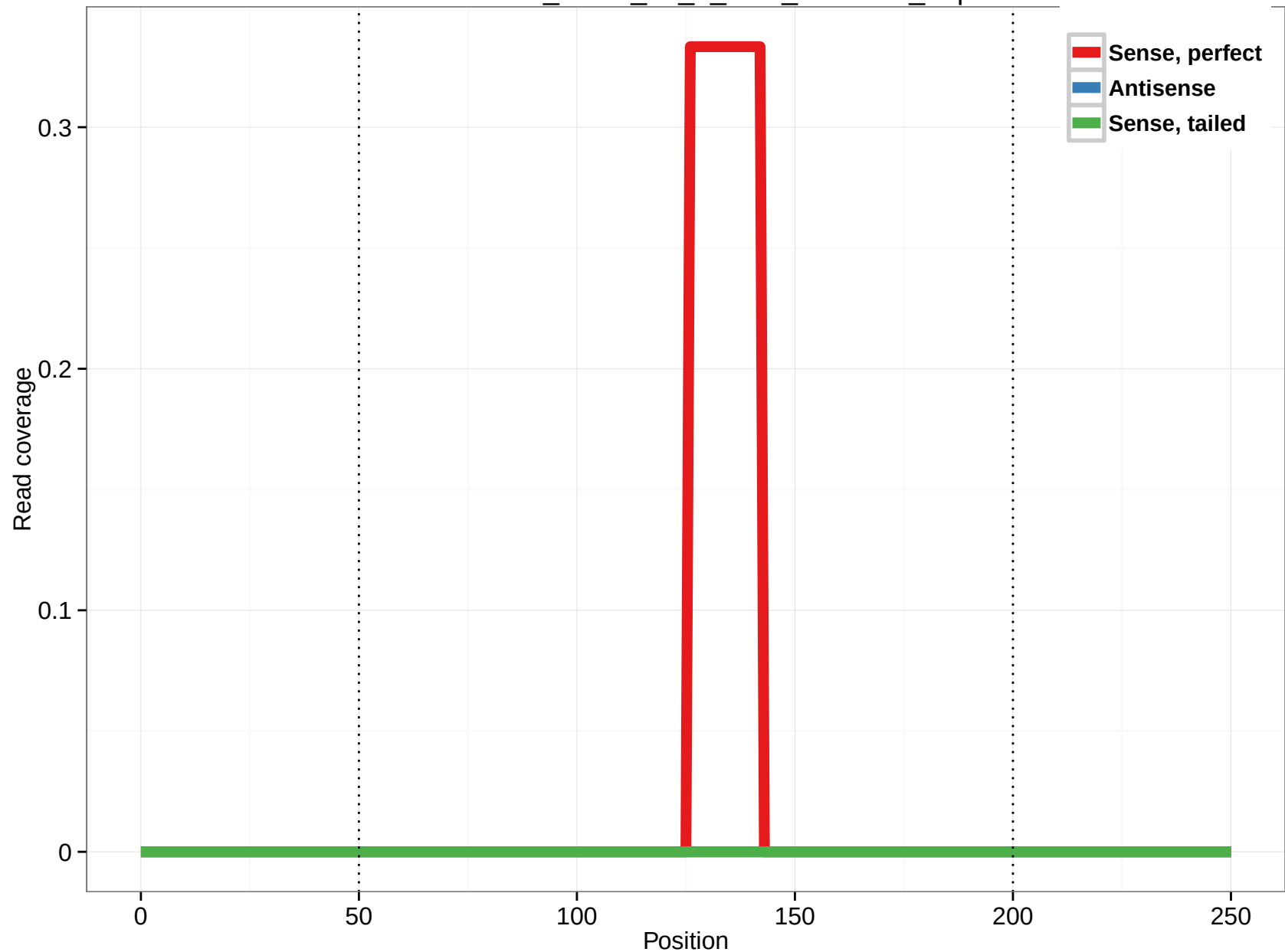
uc003zko.2_intron_13_0_chr9_8454592_r.5p
