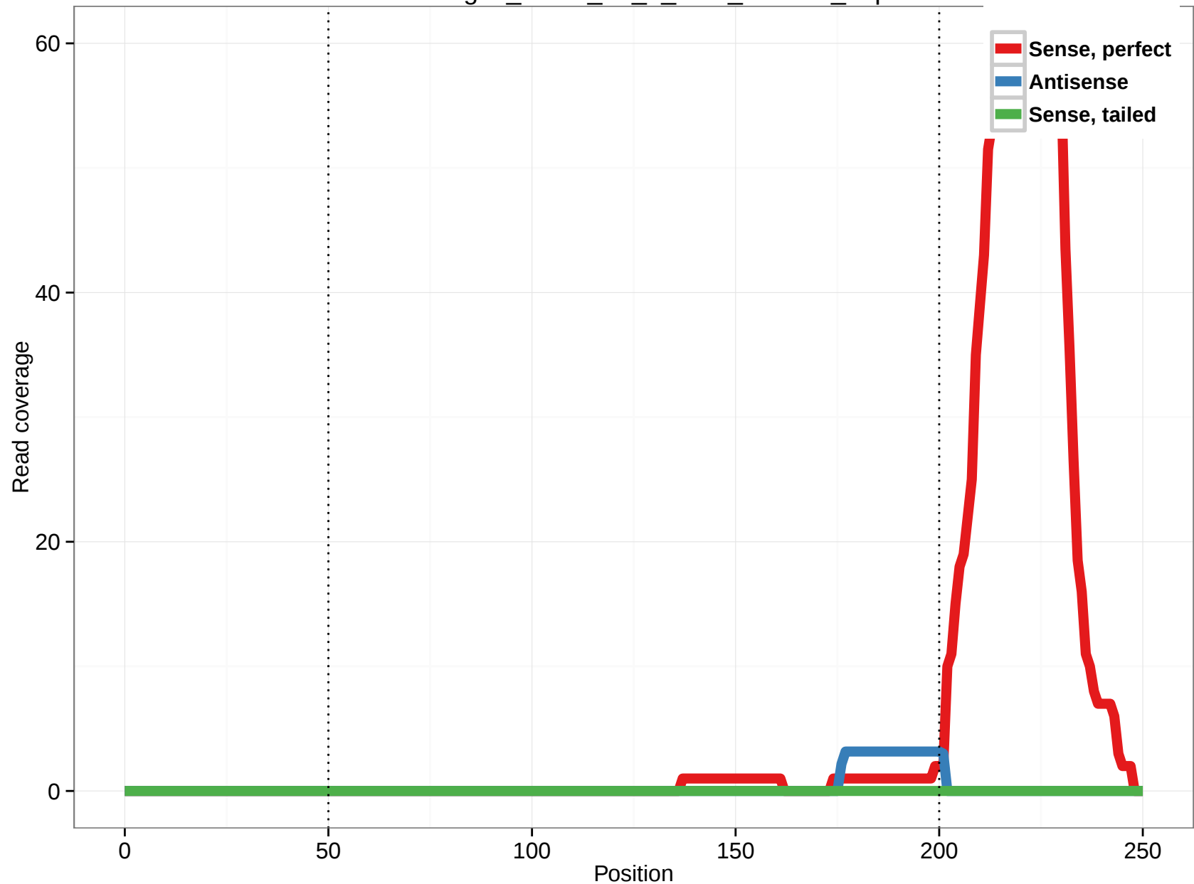
uc003zgl.1_intron_11_0_chr9_738505_f.3p
