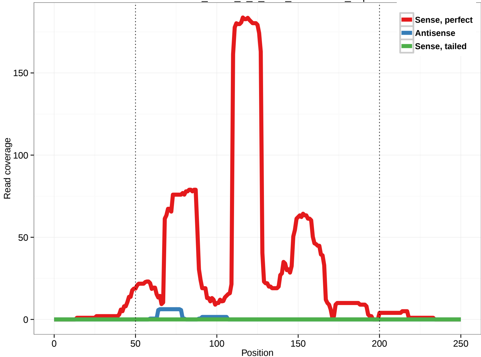
uc003zed.1_intron_0_0_chr8_146024323_f.5p
