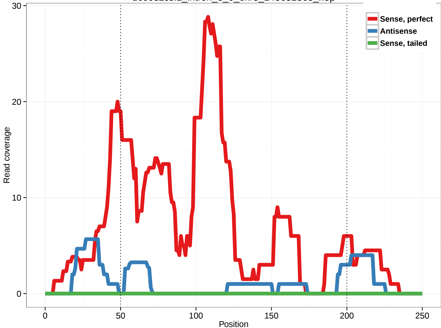
uc003zcs.1_intron_8_0_chr8_145652363_r.5p
