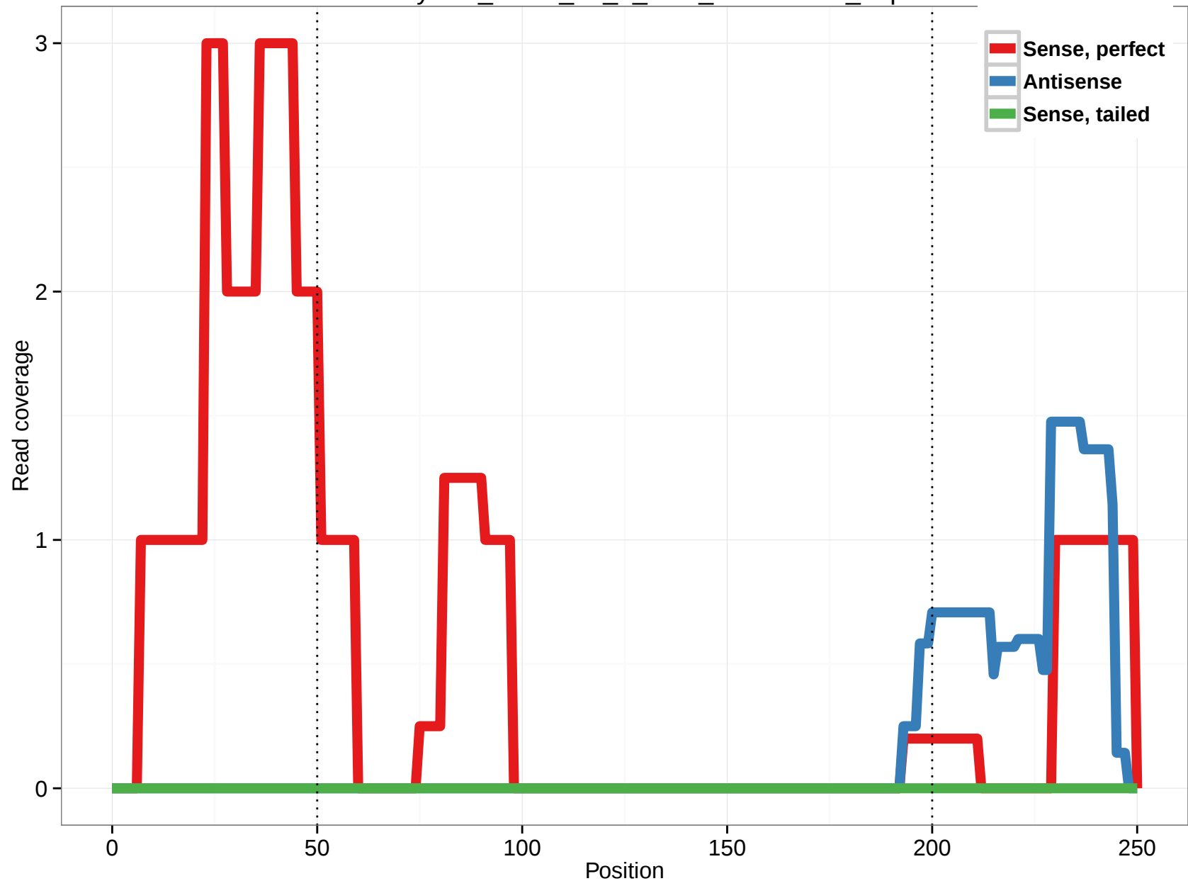
uc003yxz.2_intron_10_0_chr8_144408515_r.5p
