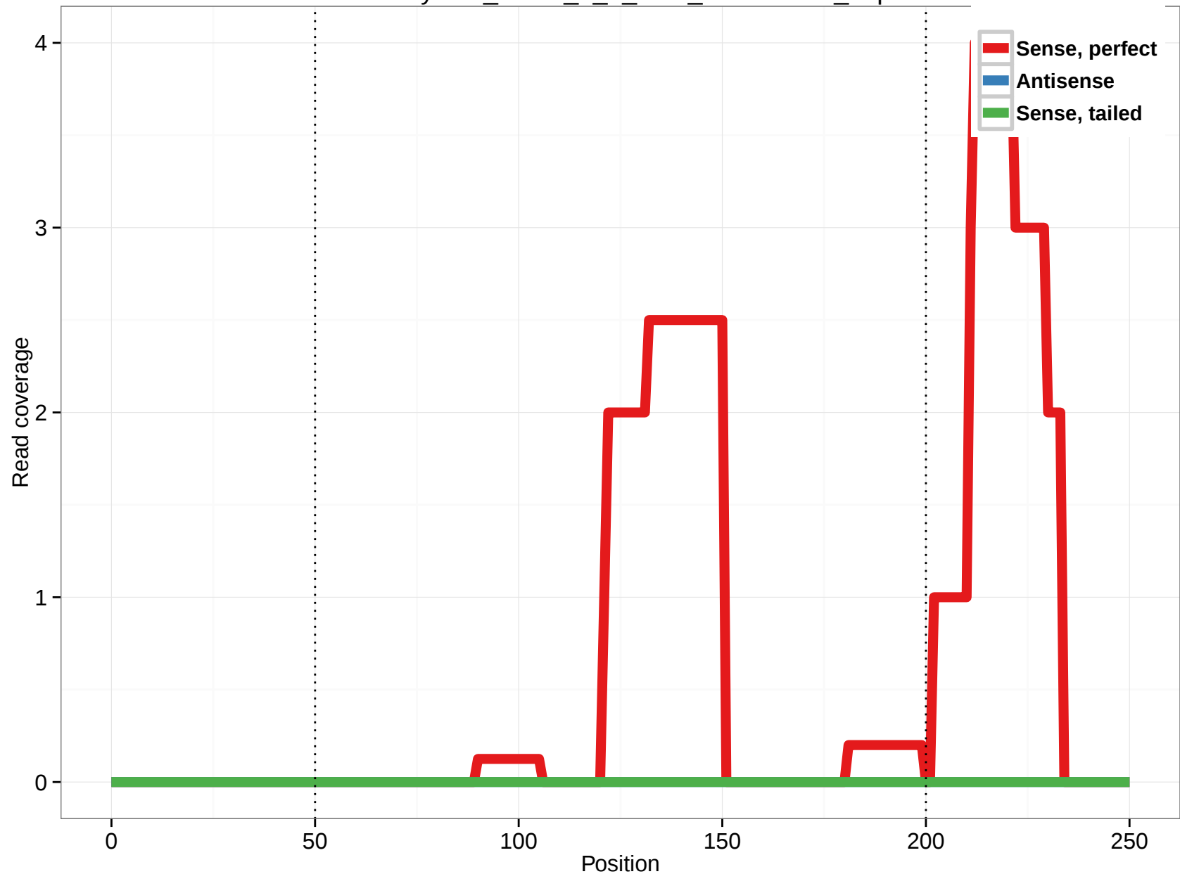
uc003yuv.2_intron_2_0_chr8_136555014_f.3p
