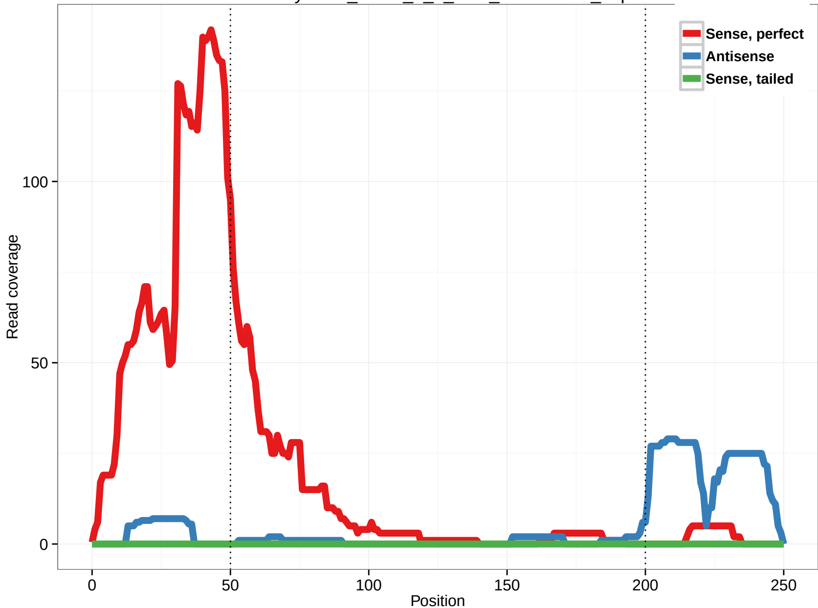
uc003ymw.1_intron_0_0_chr8_109455928_f.5p
