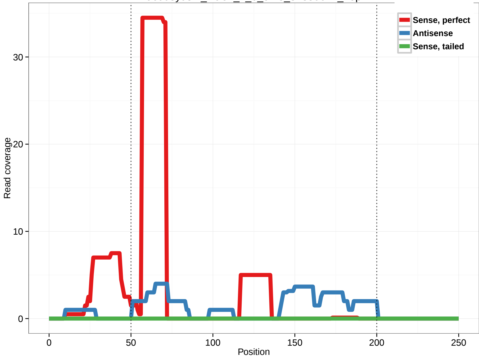
uc003yds.2_intron_2_0_chr8_87350617_r.5p
