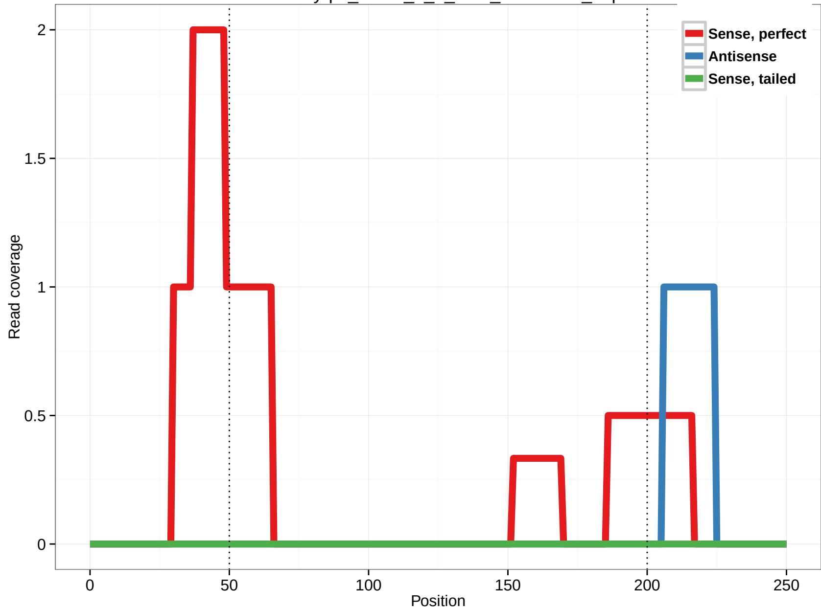
uc003xyq.2_intron_0_0_chr8_71581774_f.5p
