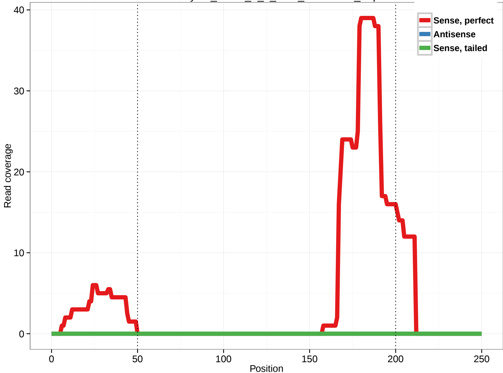
uc003xyo.1_intron_8_0_chr8_71510491_r.5p
