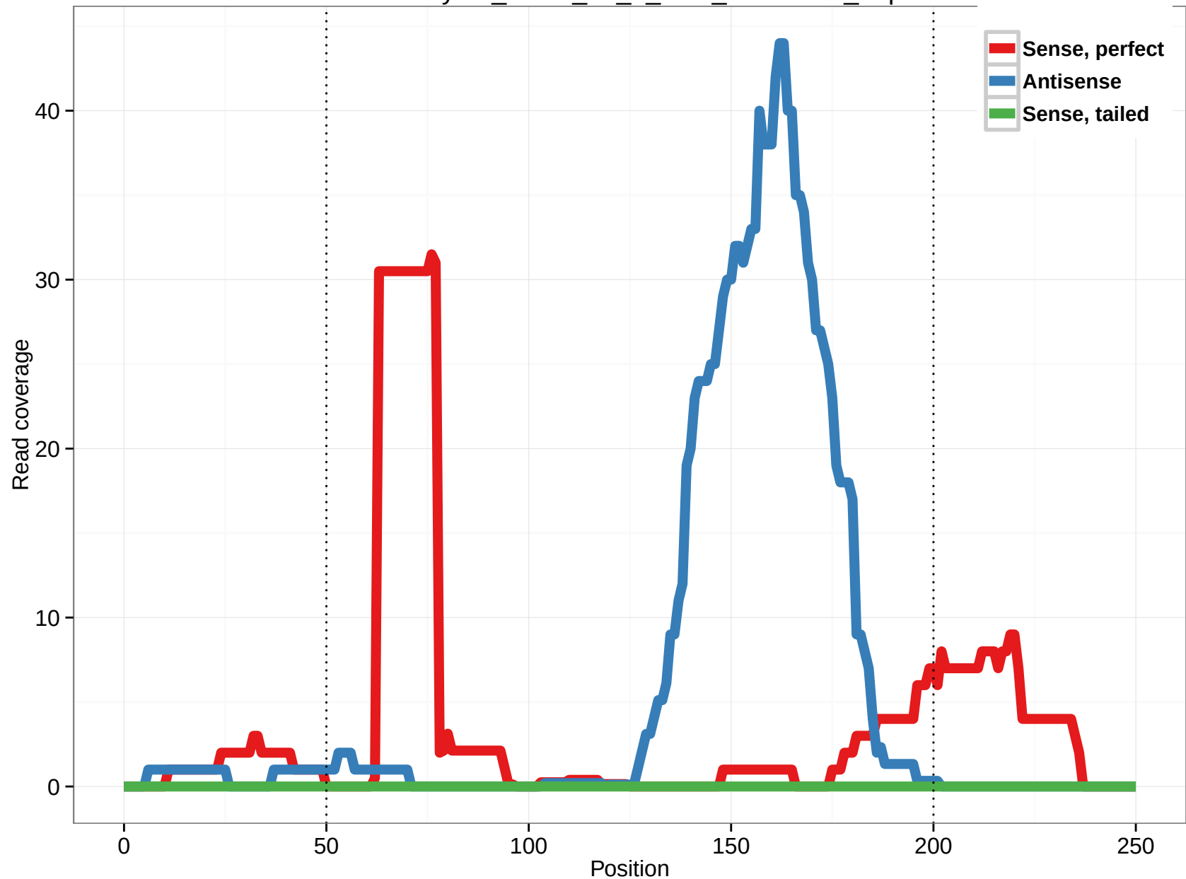
uc003xyn.1_intron_21_0_chr8_71209036_r.5p
