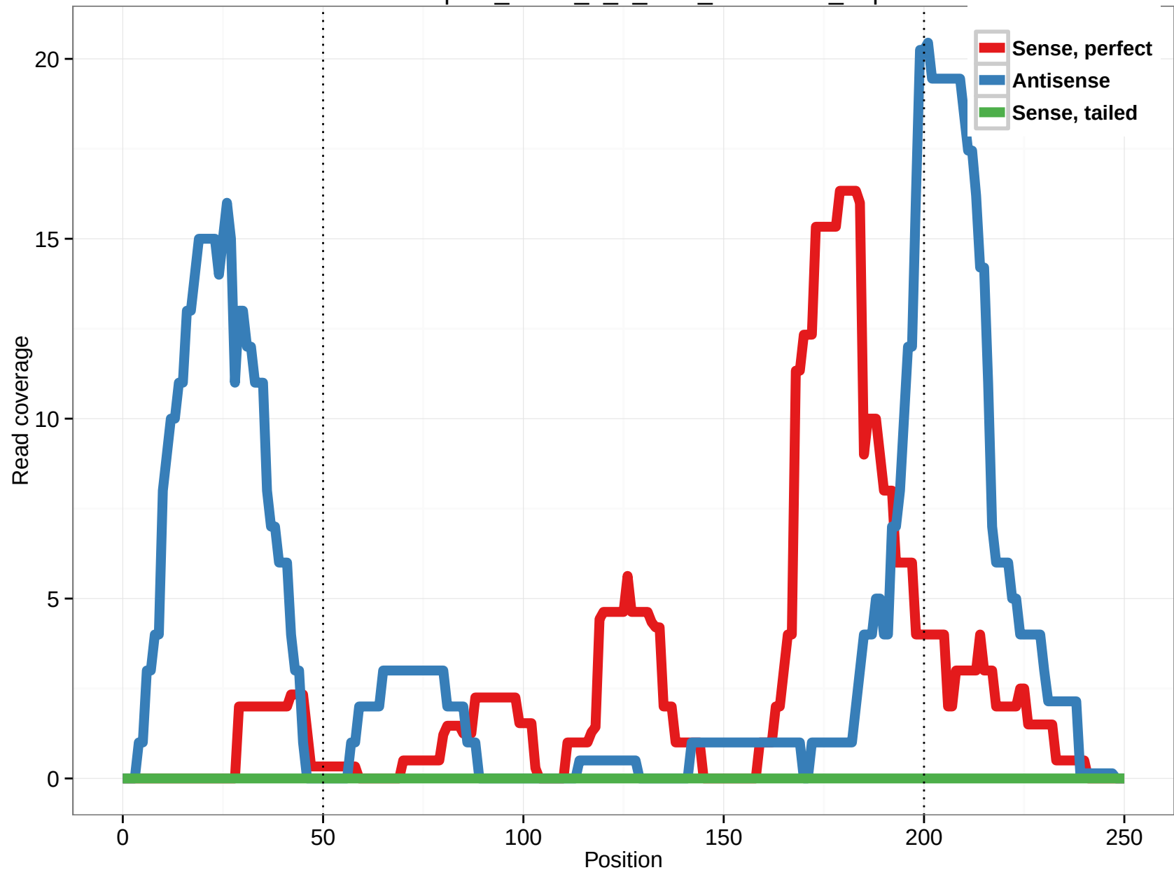
uc003xpe.2_intron_9_0_chr8_42330173_r.5p
