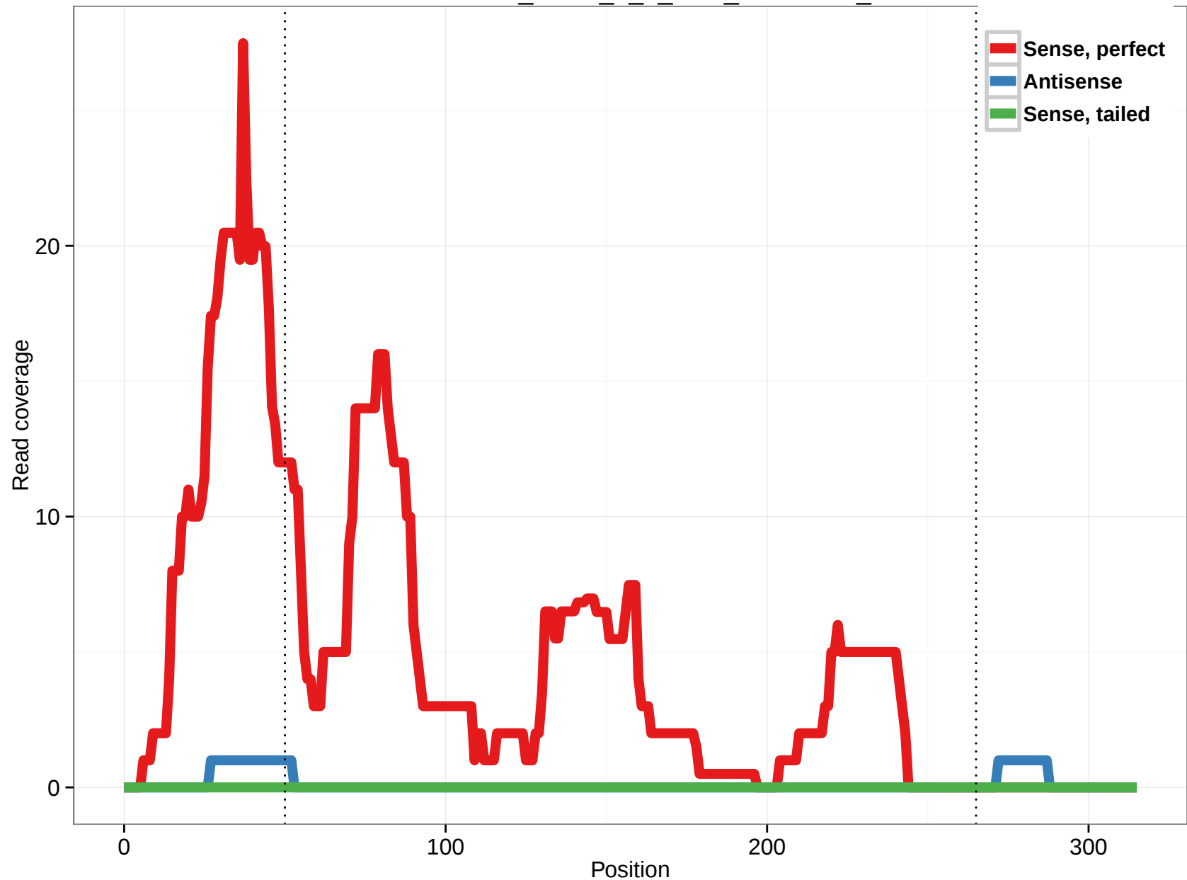
uc003xnu.2_intron_0_0_chr8_41348137_f
