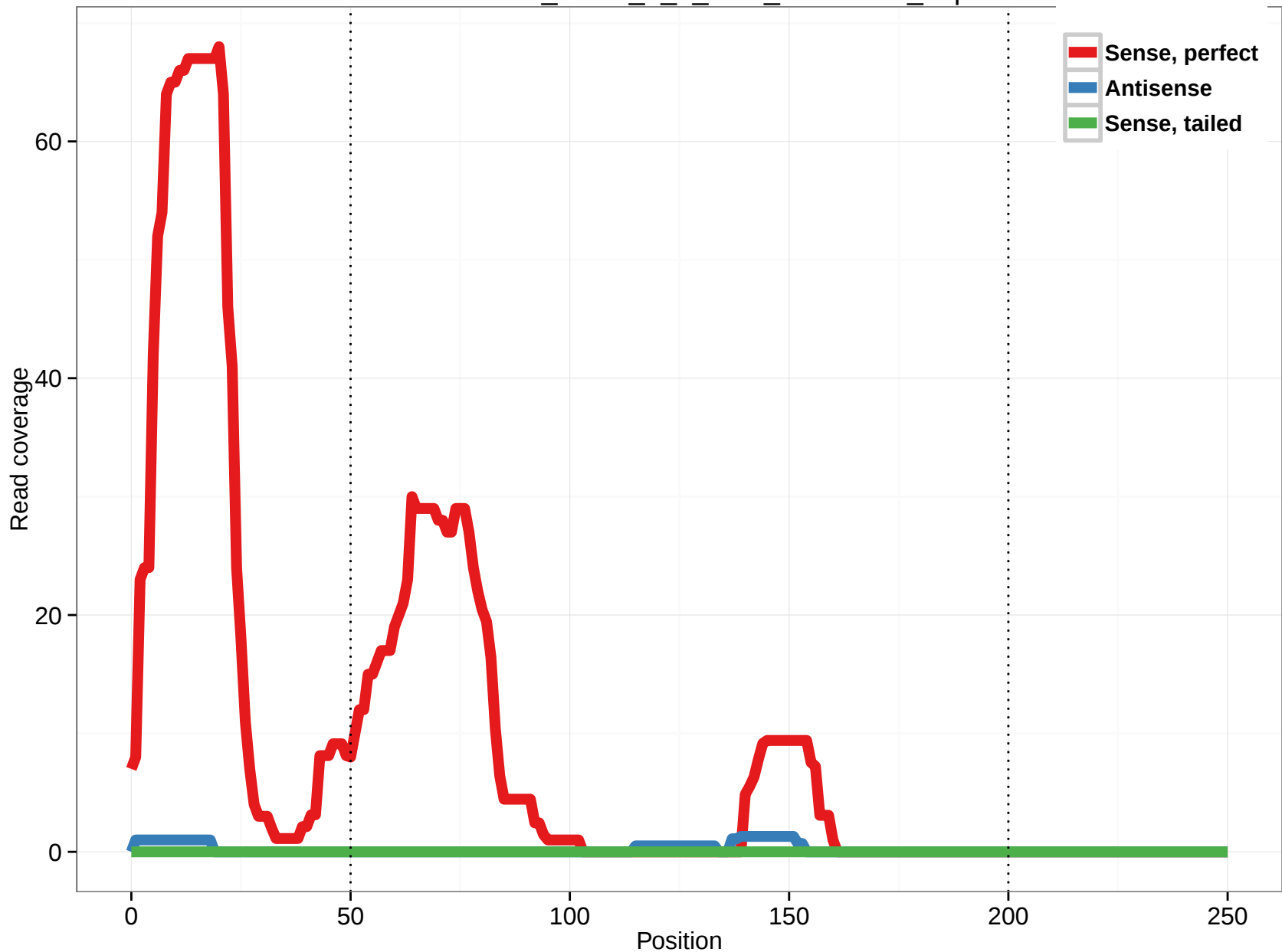
uc003xhw.3_intron_0_0_chr8_29953045_f.5p
