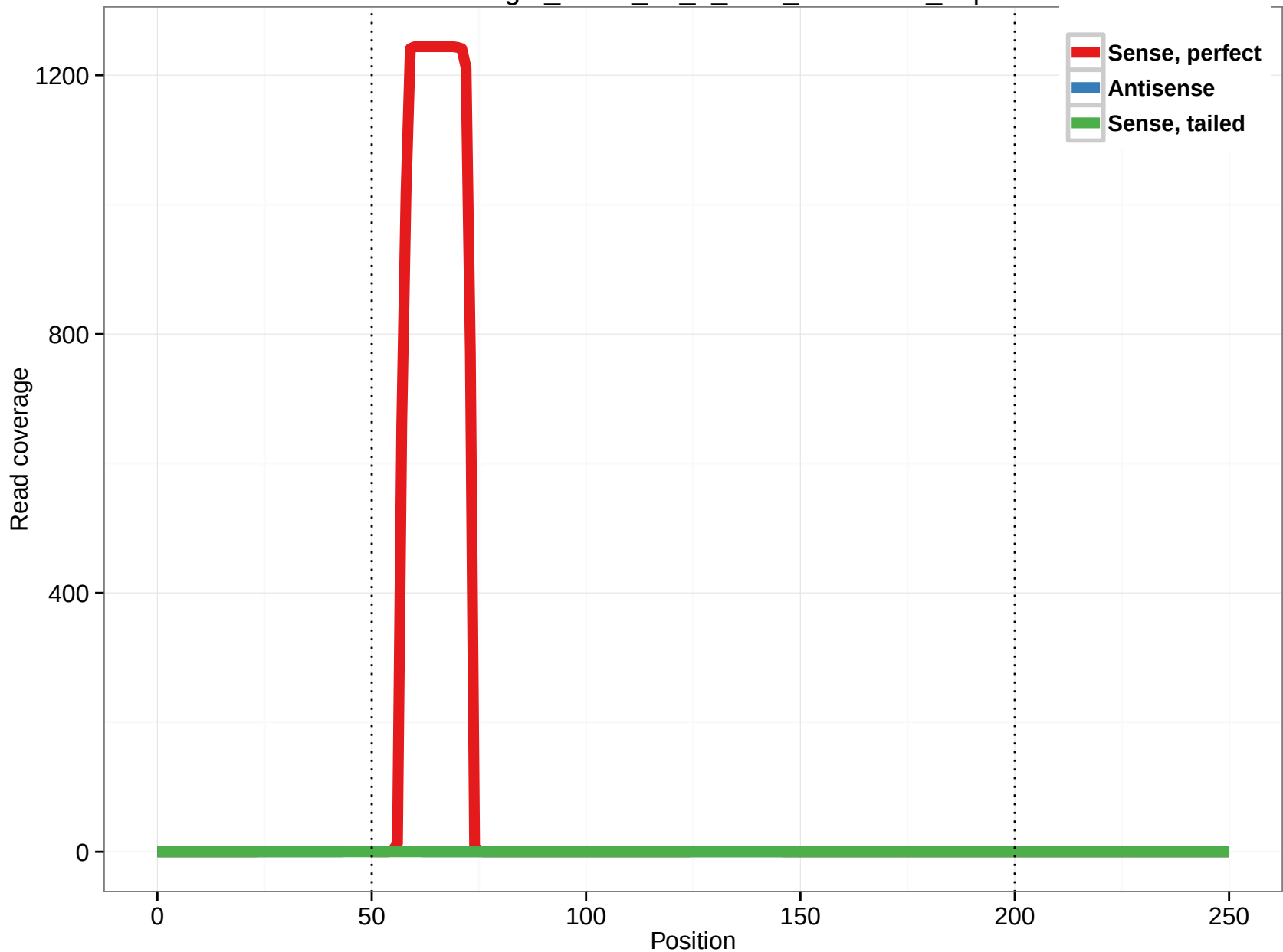
uc003xeg.2_intron_40_0_chr8_25246749_f.5p
