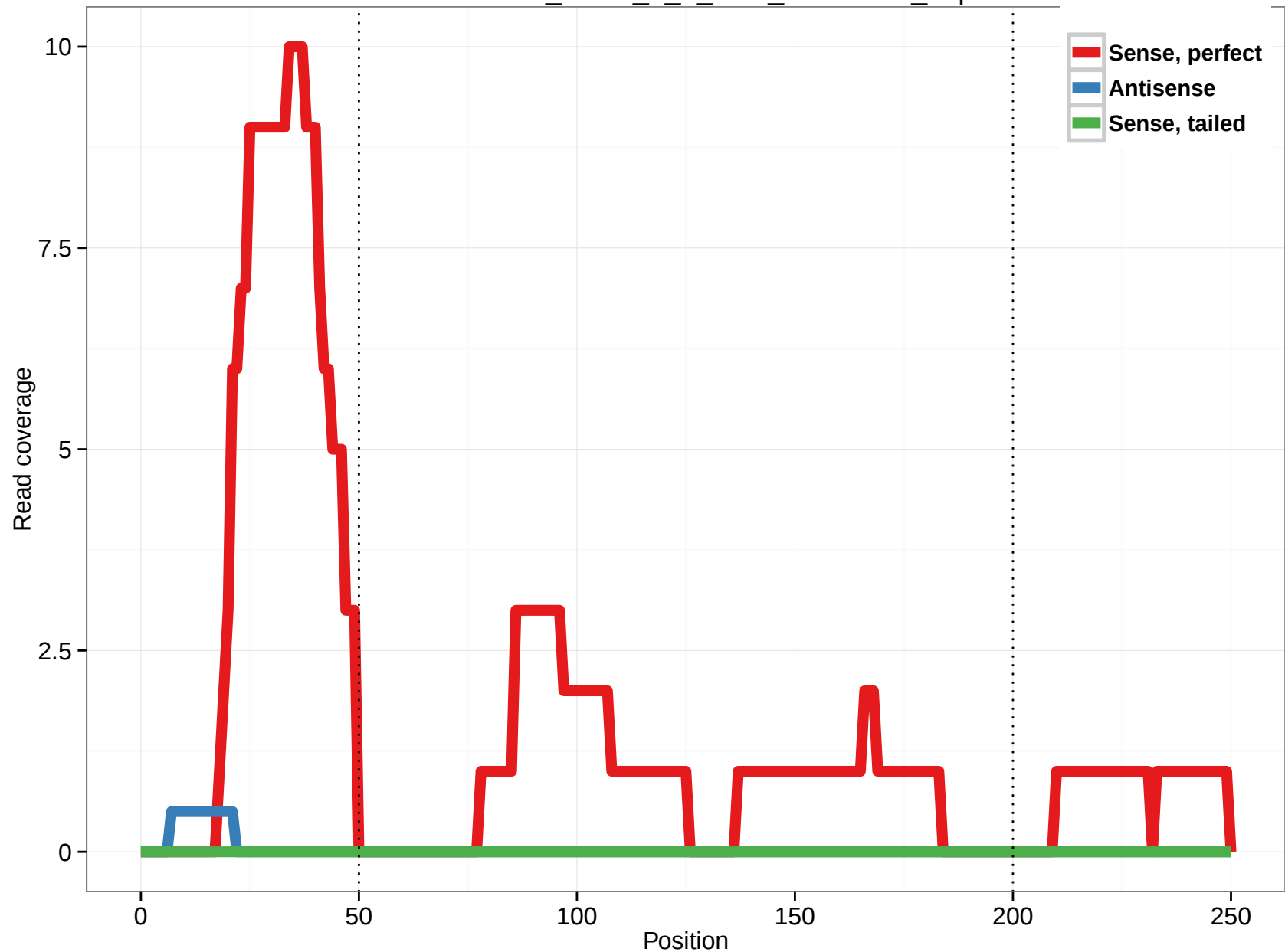
uc003xdn.1_intron_0_0_chr8_23386726_f.5p
