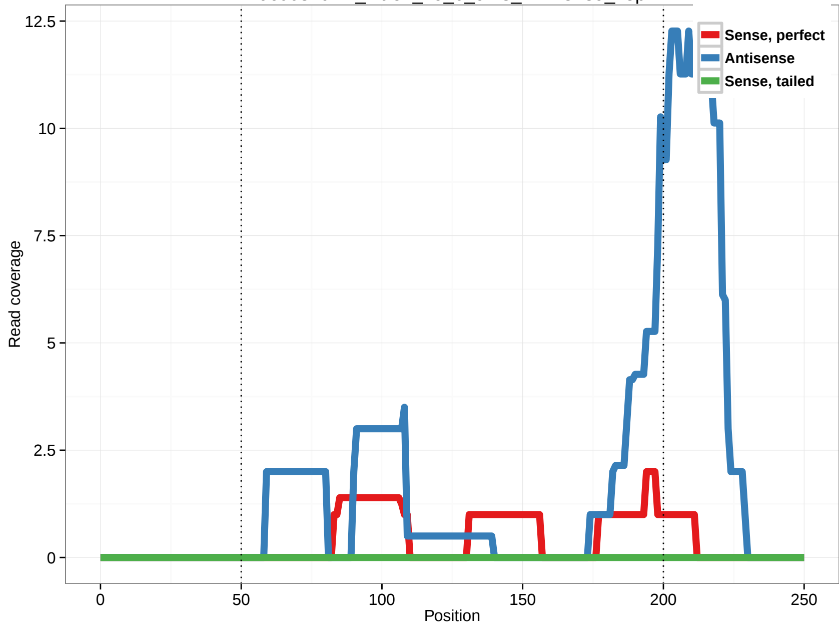
uc003xbn.2_intron_19_0_chr8_22175789_f.5p
