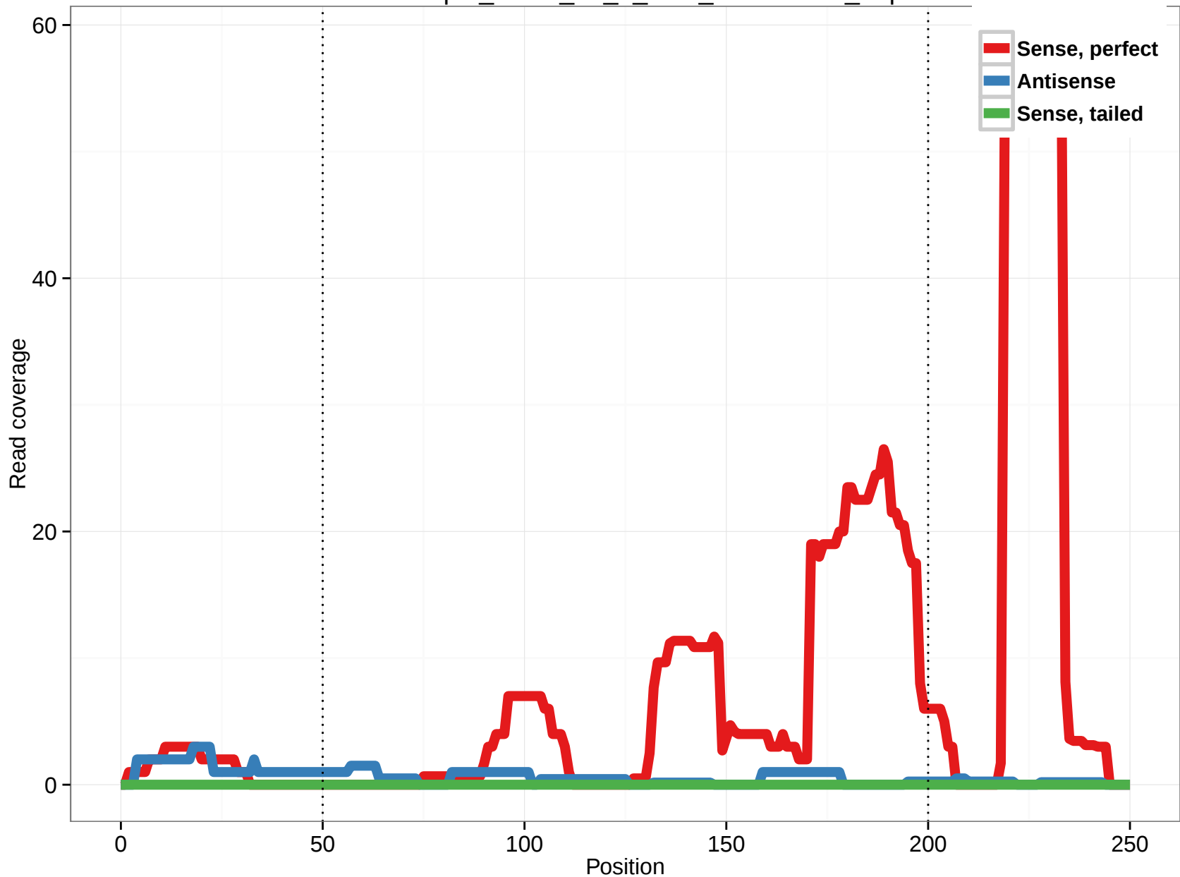
uc003wlp.2_intron_19_0_chr7_154790495_r.5p
