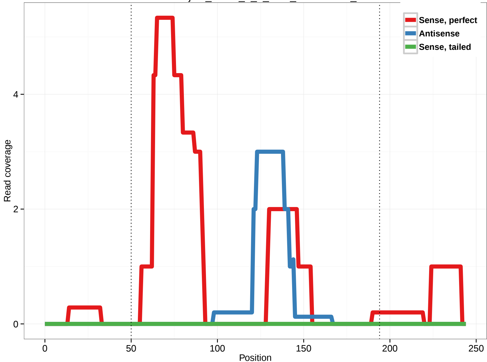
uc003wjb.2_intron_7_0_chr7_151058001_f
