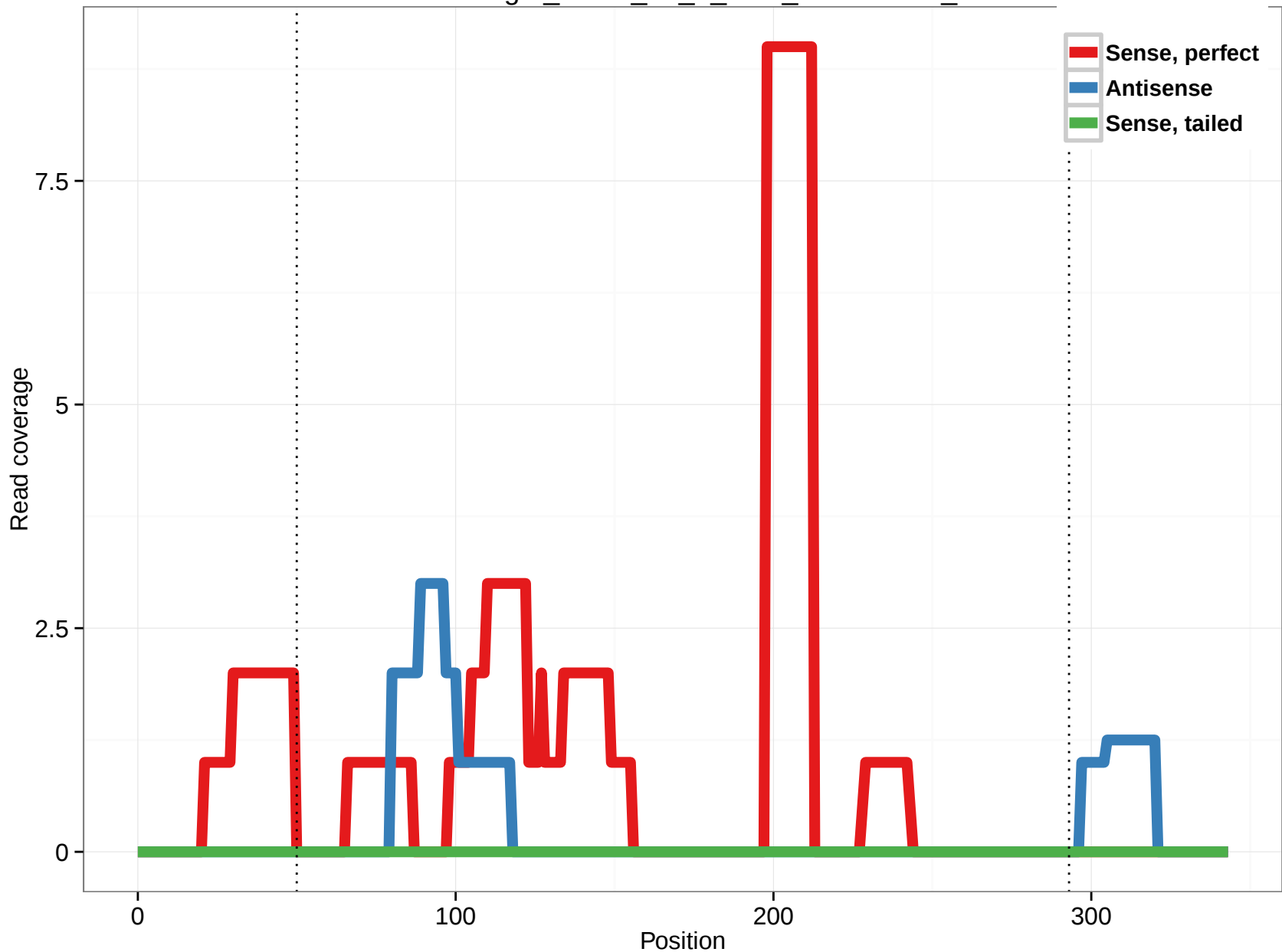
uc003wig.3_intron_10_0_chr7_150715138_r
