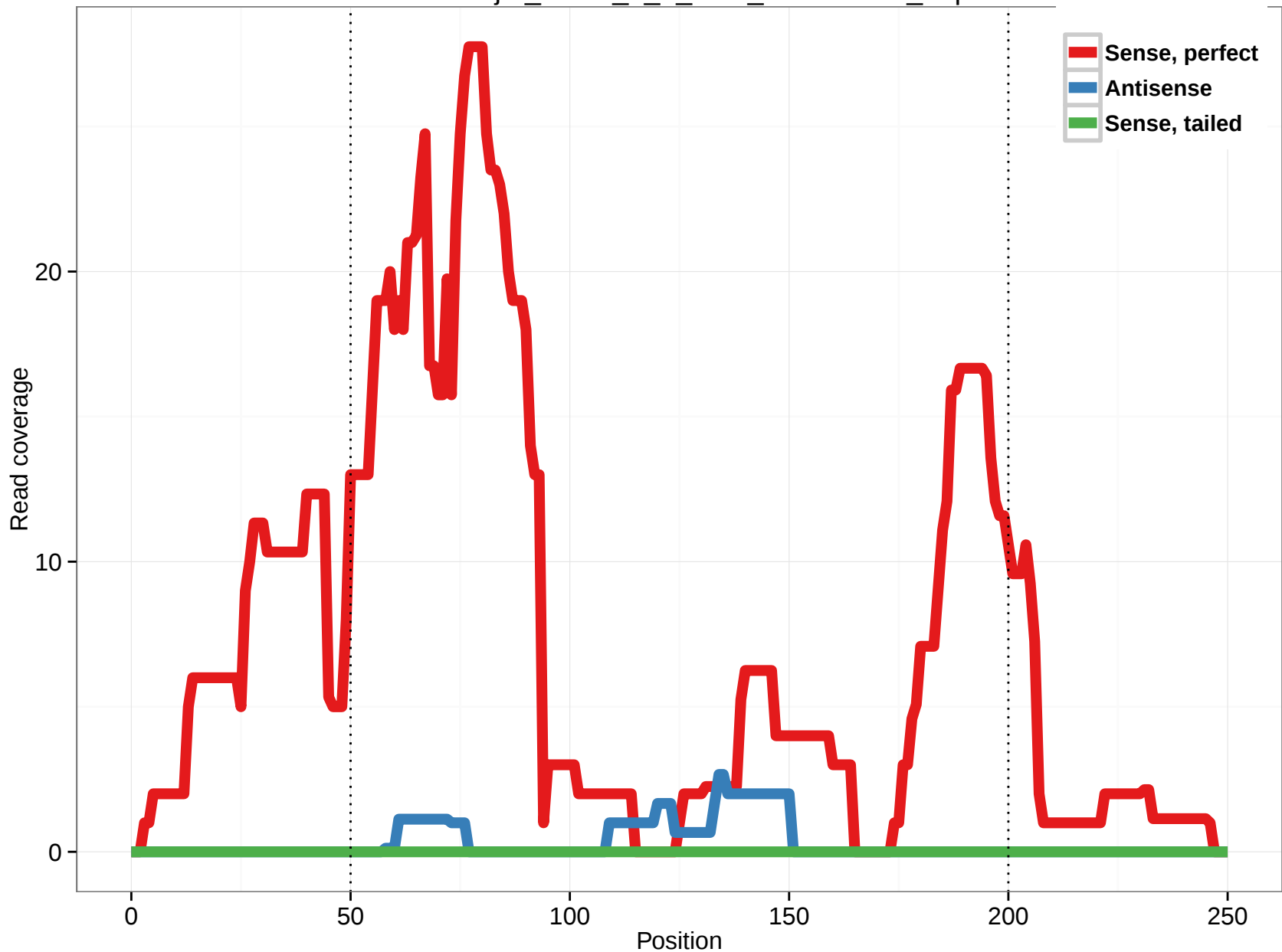
uc003wfj.2_intron_2_0_chr7_148815441_r.5p
