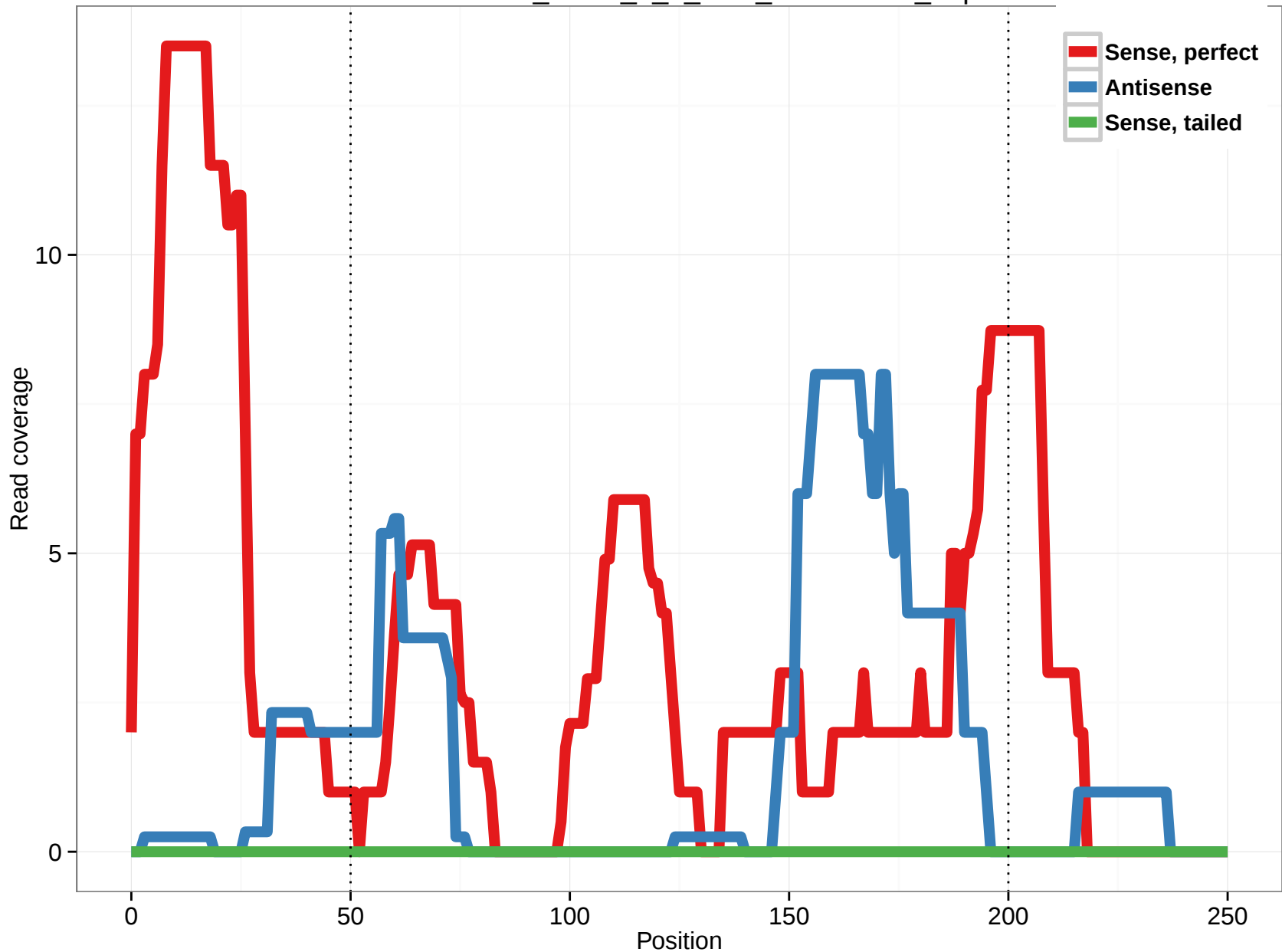
uc003wdo.1_intron_7_0_chr7_143573716_r.5p
