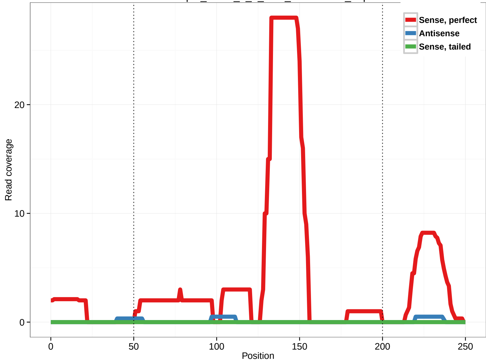
uc003vrp.1_intron_2_0_chr7_134132134_r.3p
