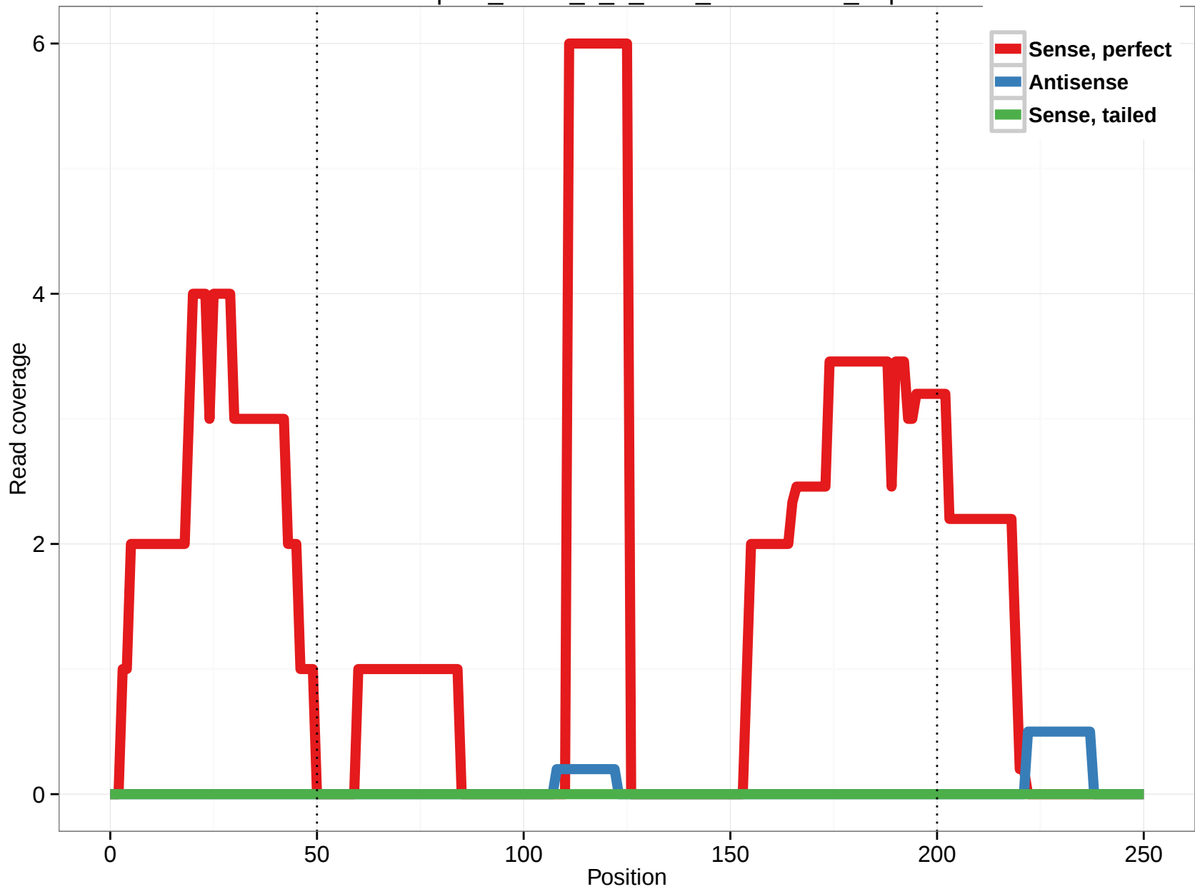
uc003vph.2_intron_6_0_chr7_129679388_r.5p
