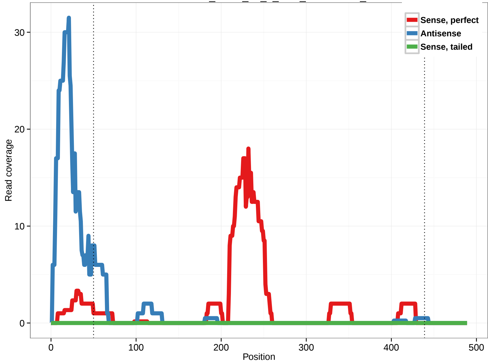
uc003vmw.2_intron_14_0_chr7_128049421_r
