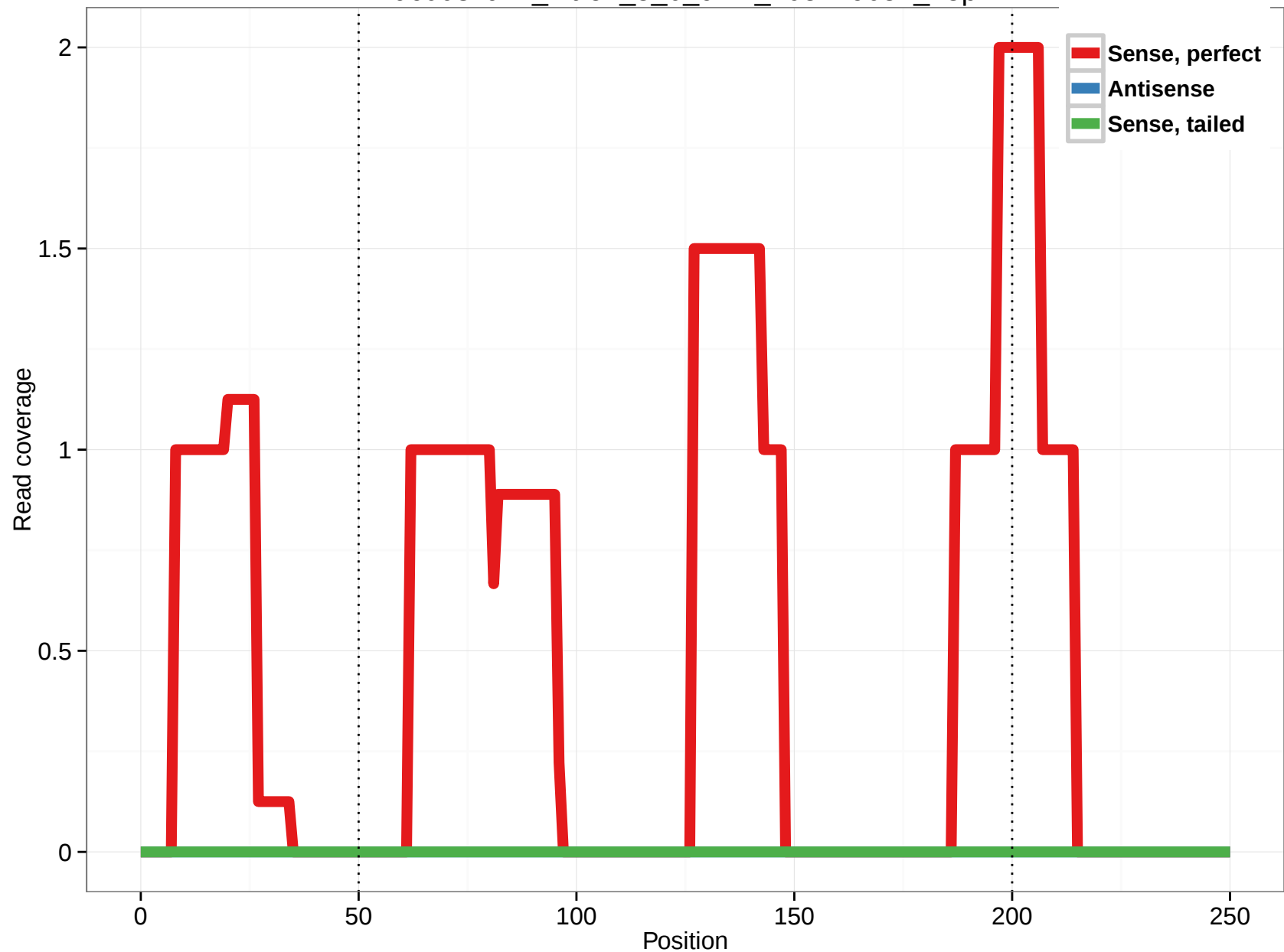
uc003vdf.2_intron_5_0_chr7_105279057_r.5p
