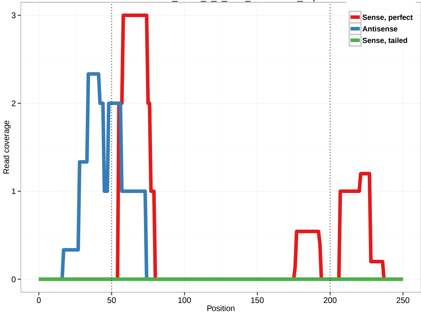
uc003vda.1_intron_1_0_chr7_105173317_f.3p
