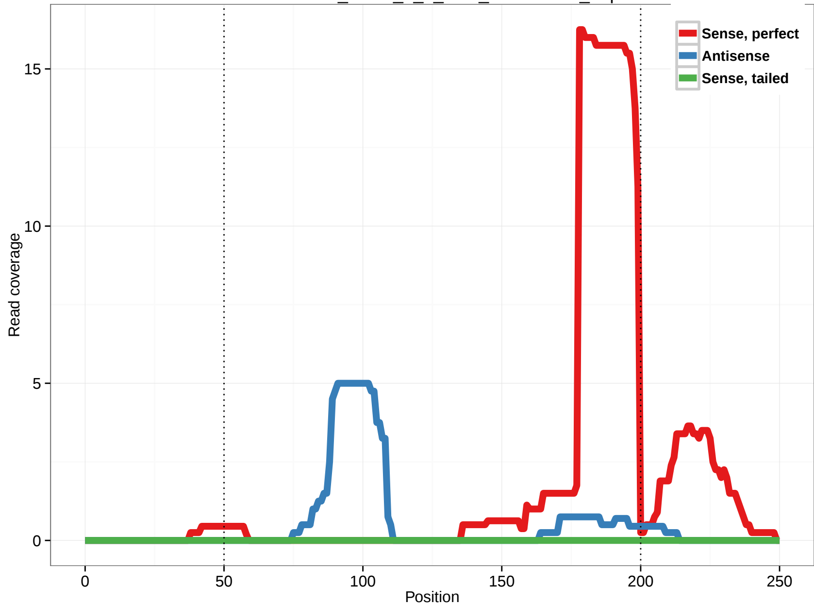
uc003vad.2_intron_5_0_chr7_102233586_r.3p
