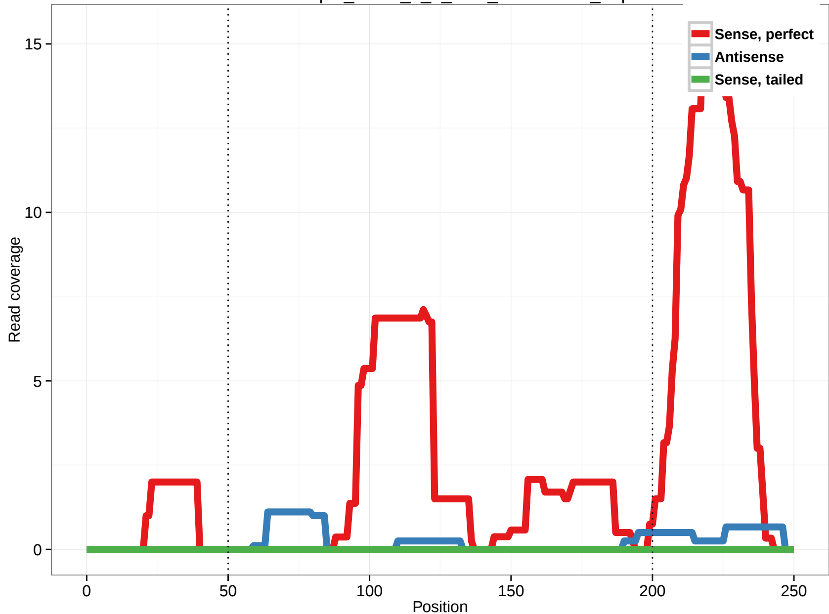
uc003uzp.1_intron_2_0_chr7_102116718_r.3p
