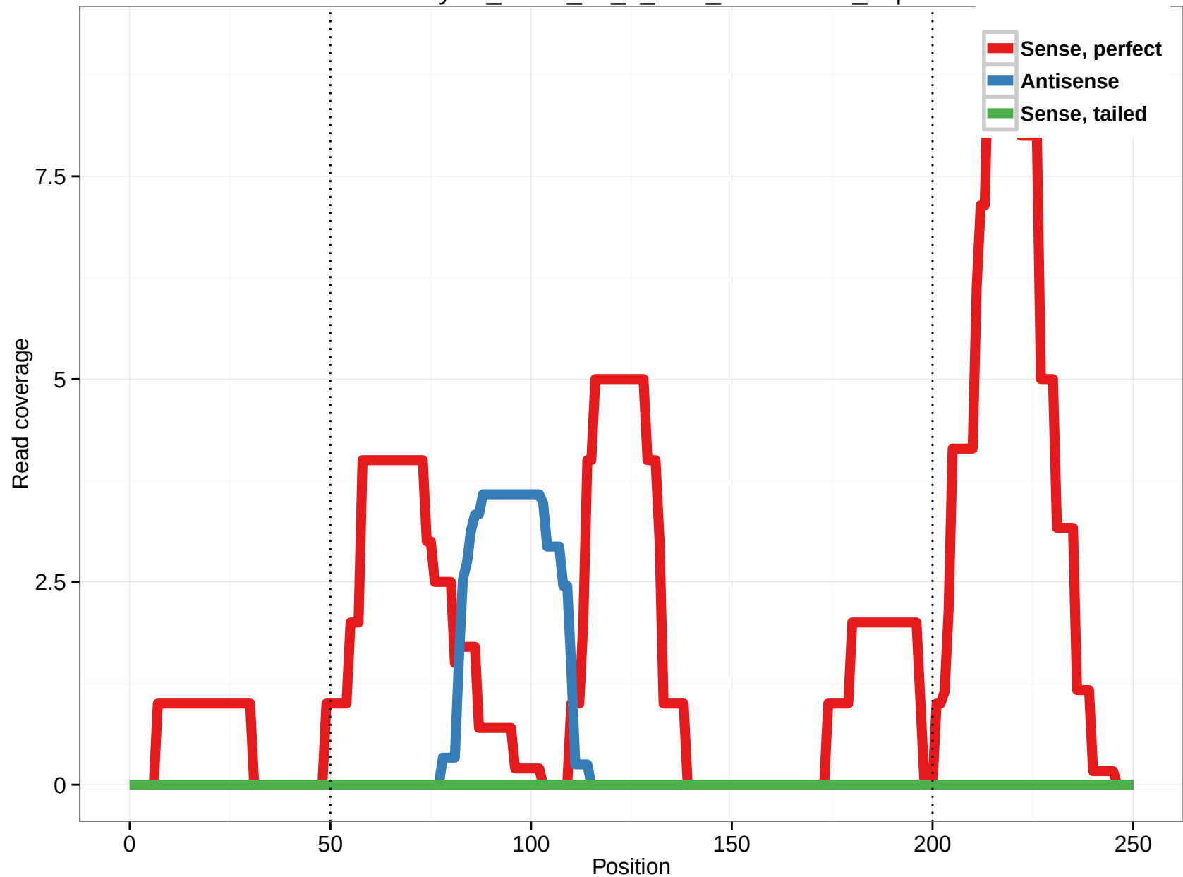
uc003uys.3_intron_11_0_chr7_101833152_f.3p
