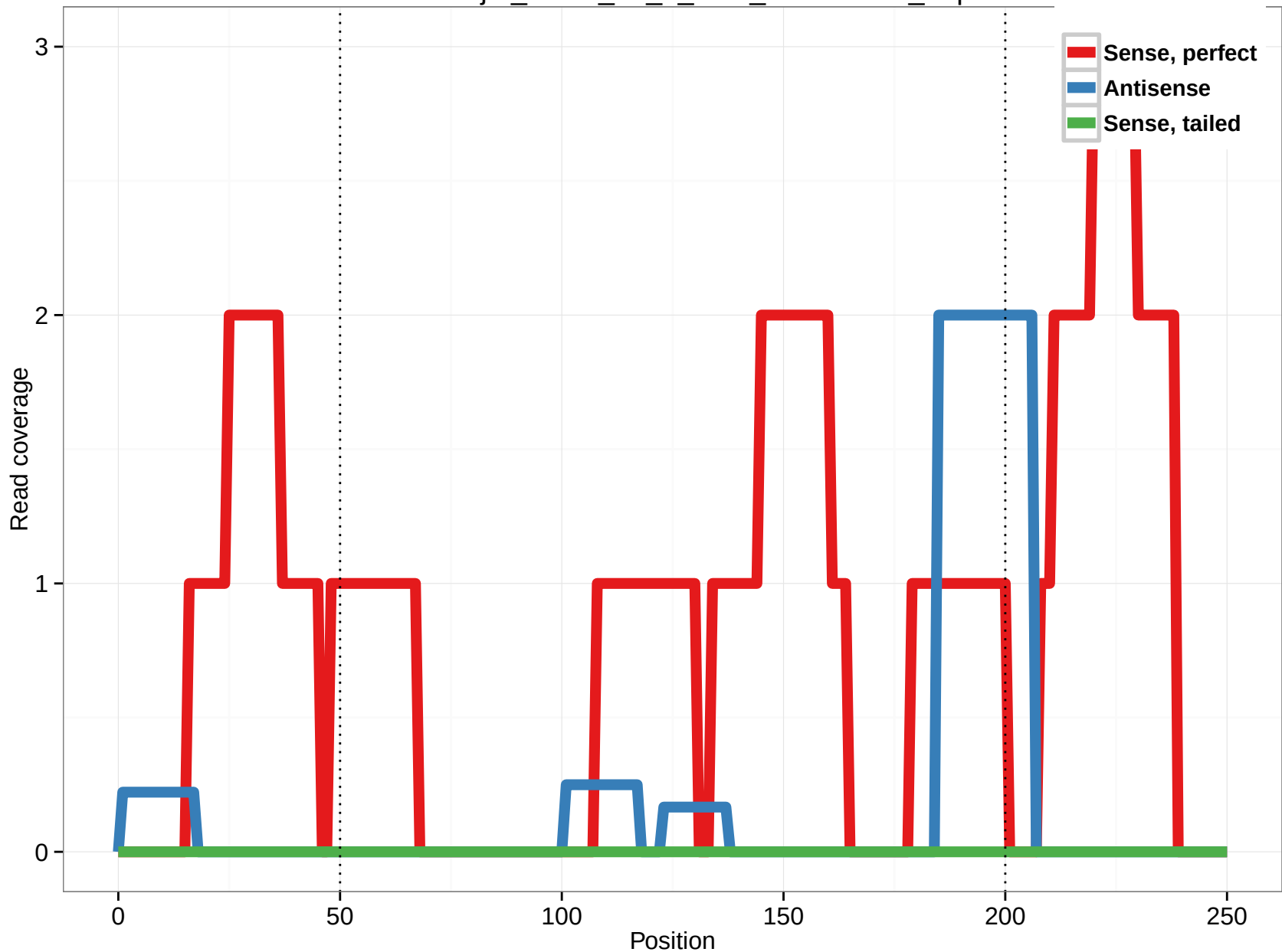
uc003uvj.2_intron_16_0_chr7_100180083_r.3p
