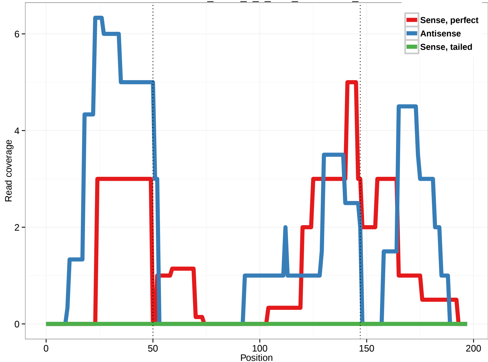
uc003uux.1_intron_0_0_chr7_100033157_r
