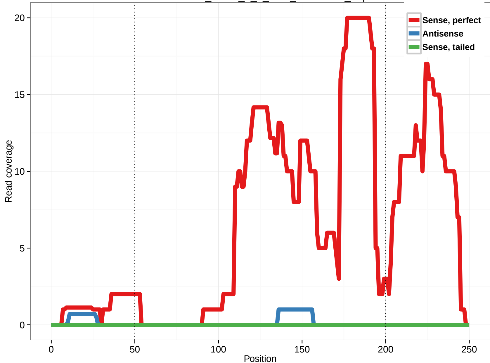
uc003uih.2_intron_8_0_chr7_86810658_f.3p
