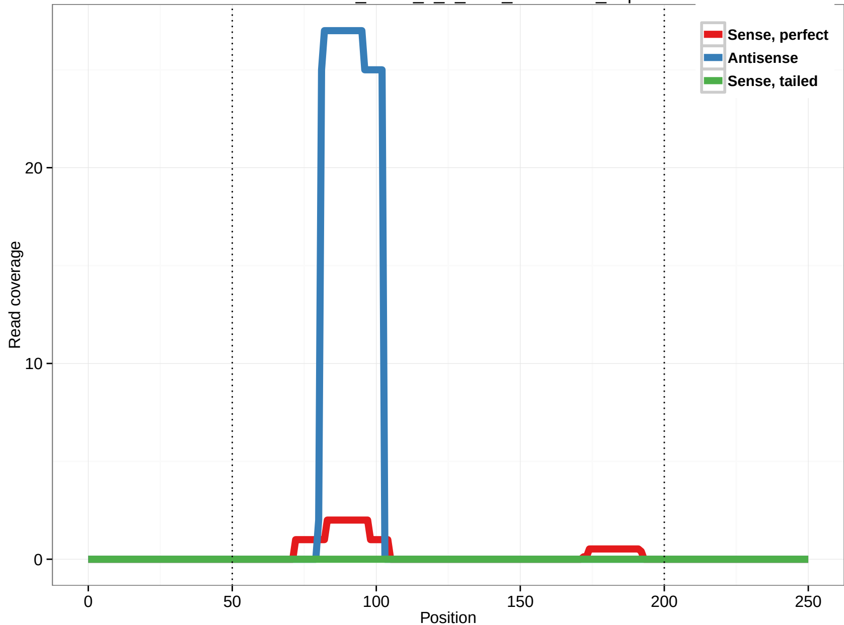
uc003uhx.2_intron_3_0_chr7_82430908_r.3p
