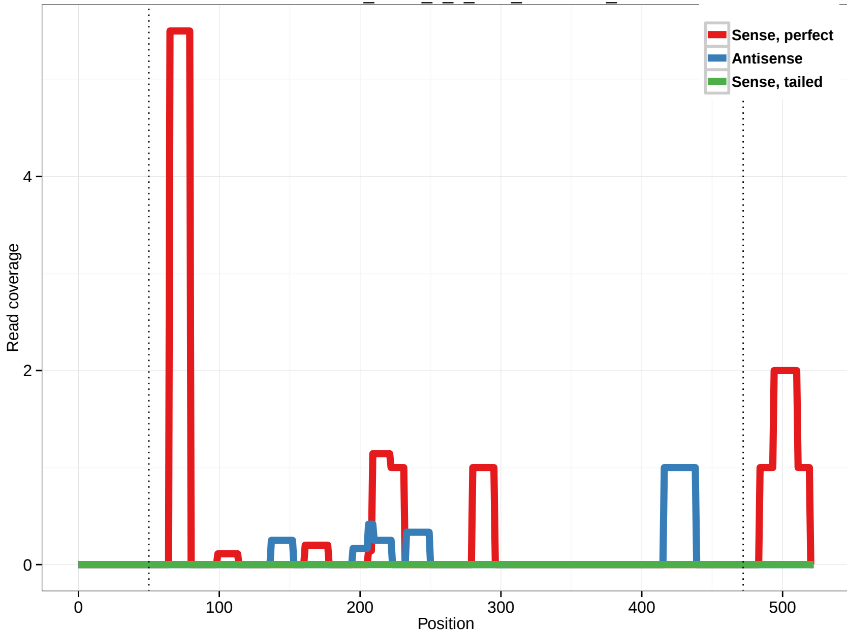
uc003uet.1_intron_1_0_chr7_75912420_f
