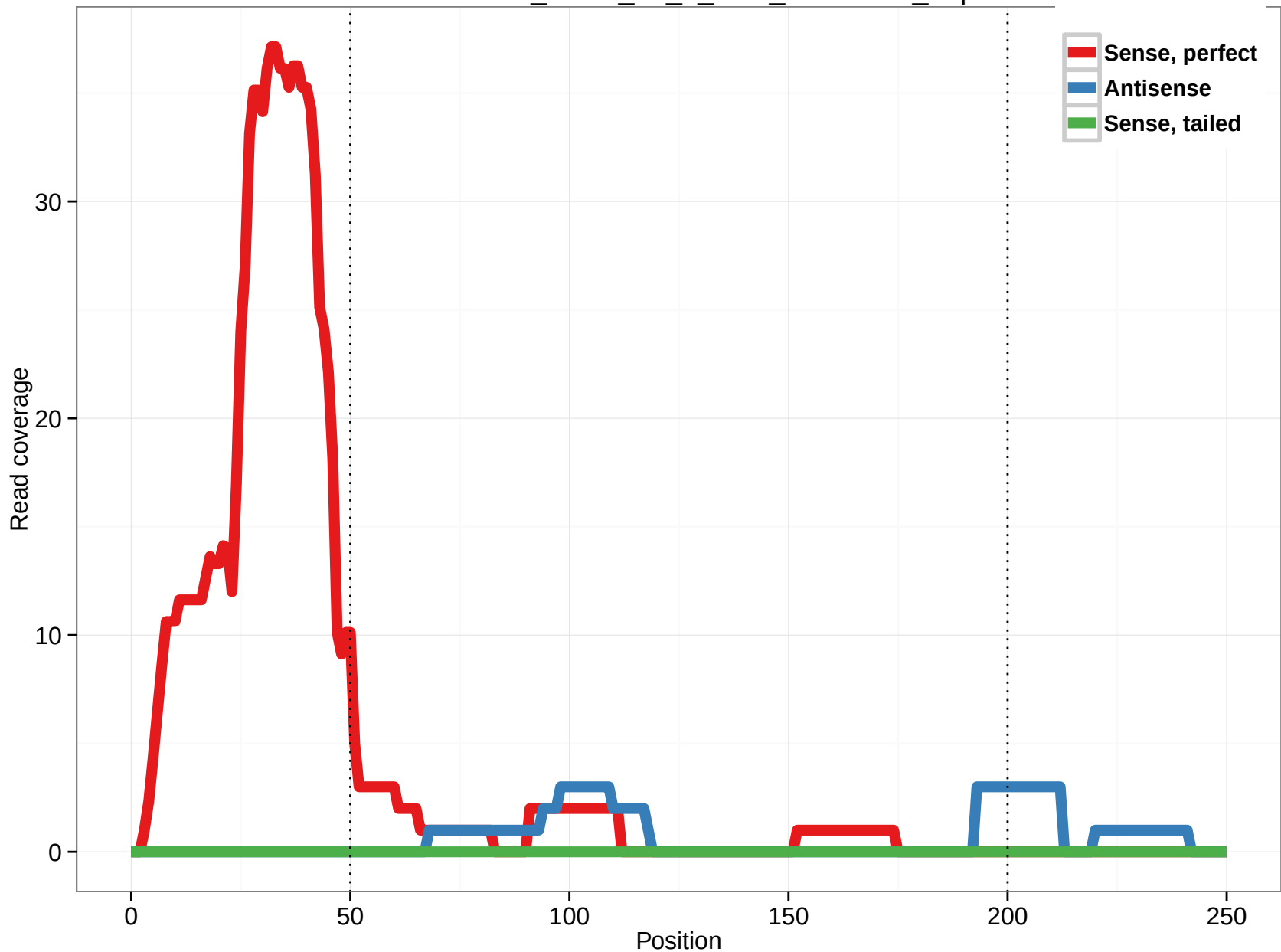
uc003ued.2_intron_11_0_chr7_75621876_r.5p
