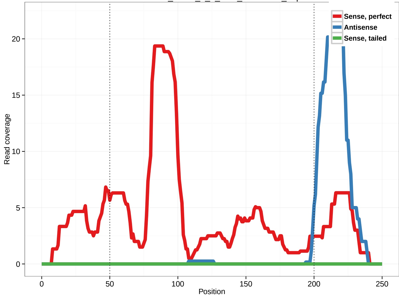
uc003ucx.2_intron_3_0_chr7_74996208_f.5p
