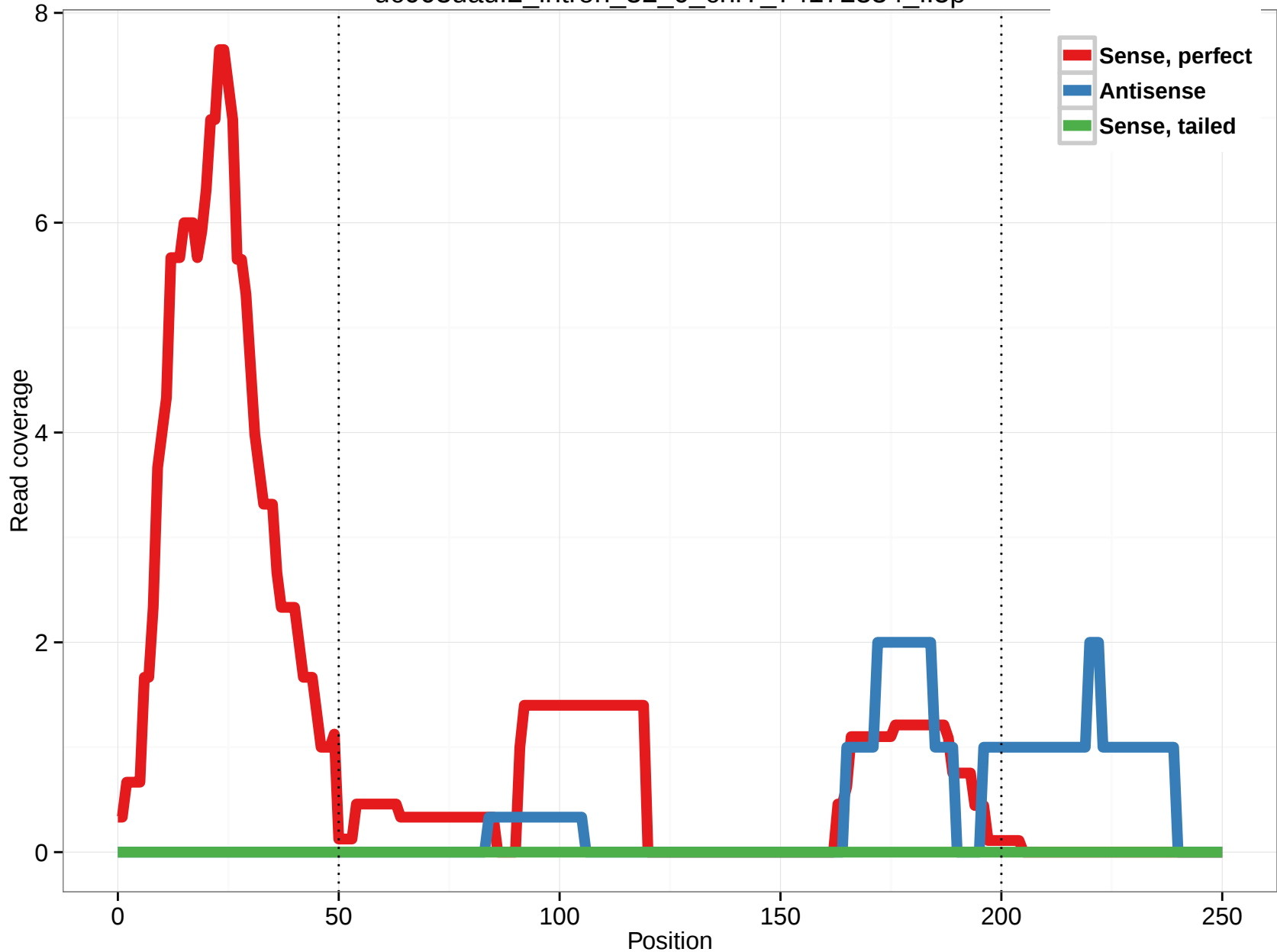
uc003uau.2_intron_32_0_chr7_74172334_f.5p
