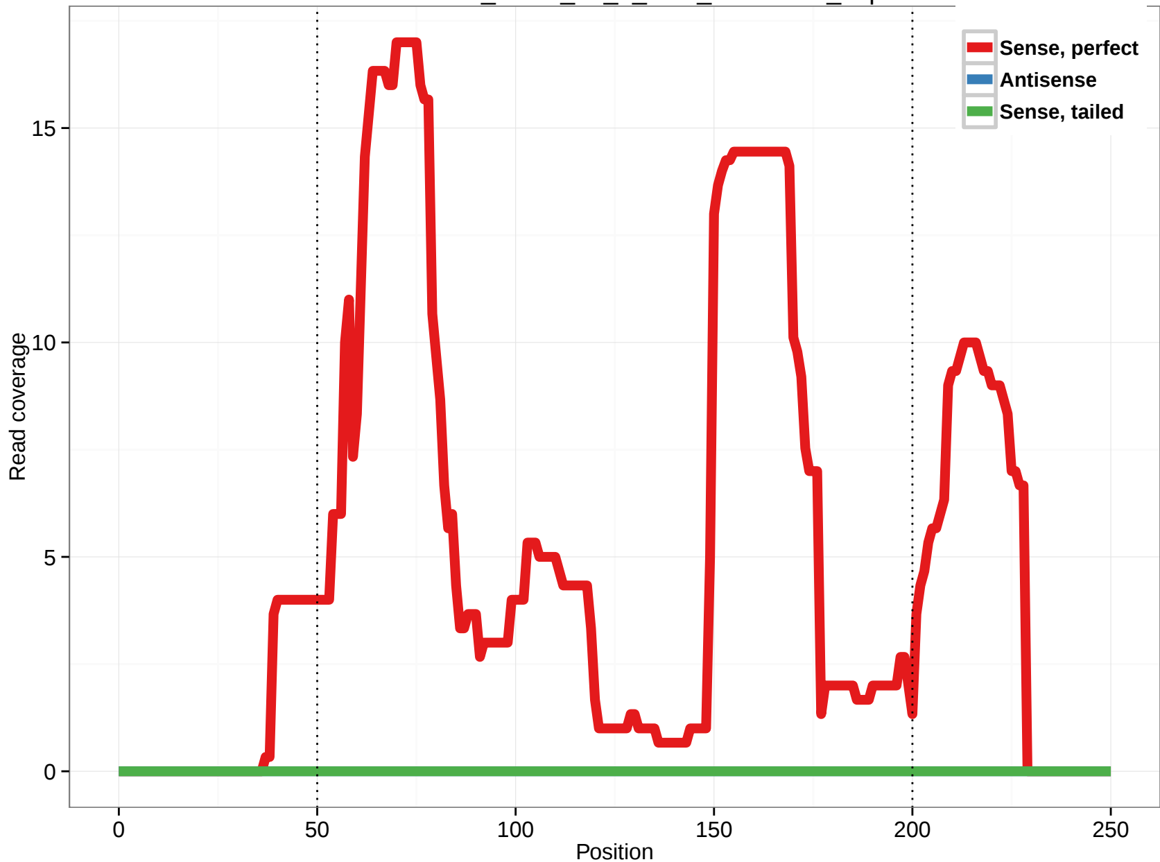
uc003uau.2_intron_29_0_chr7_74168362_f.3p
