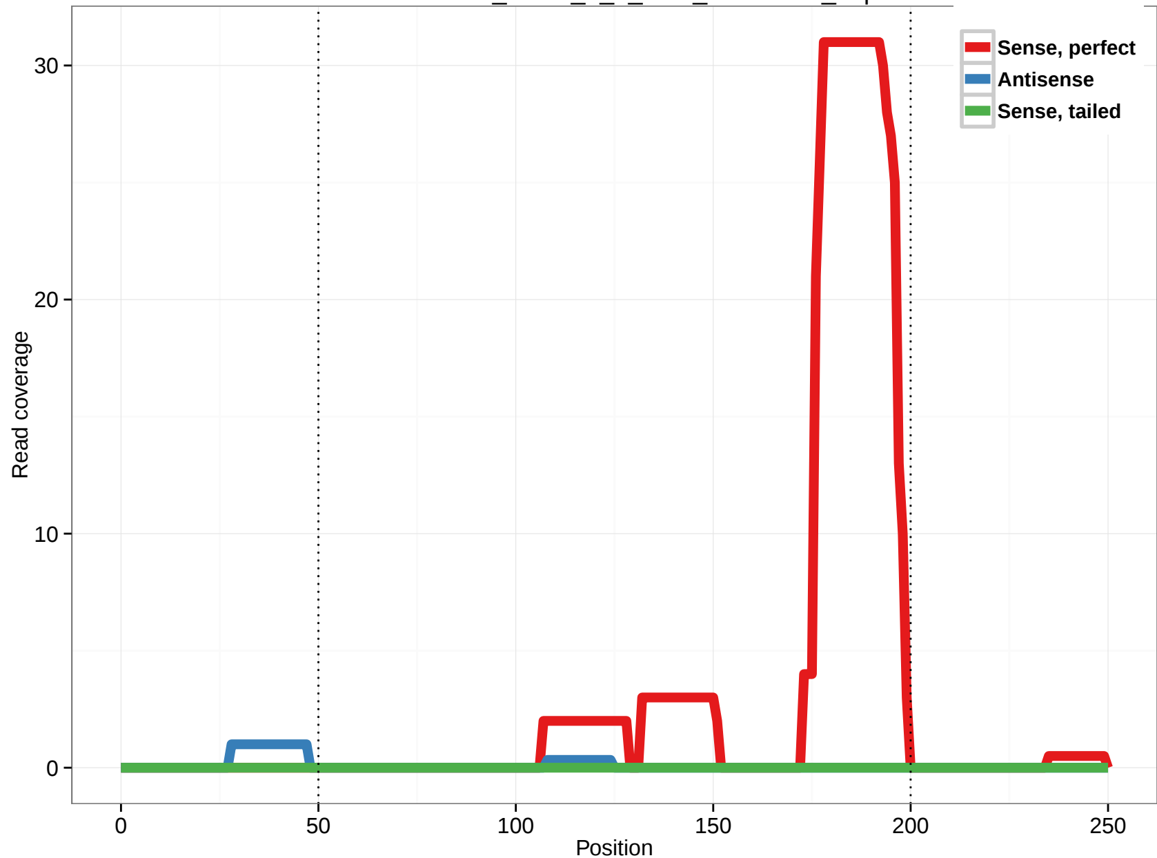
uc003uam.2_intron_3_0_chr7_73768335_f.3p
