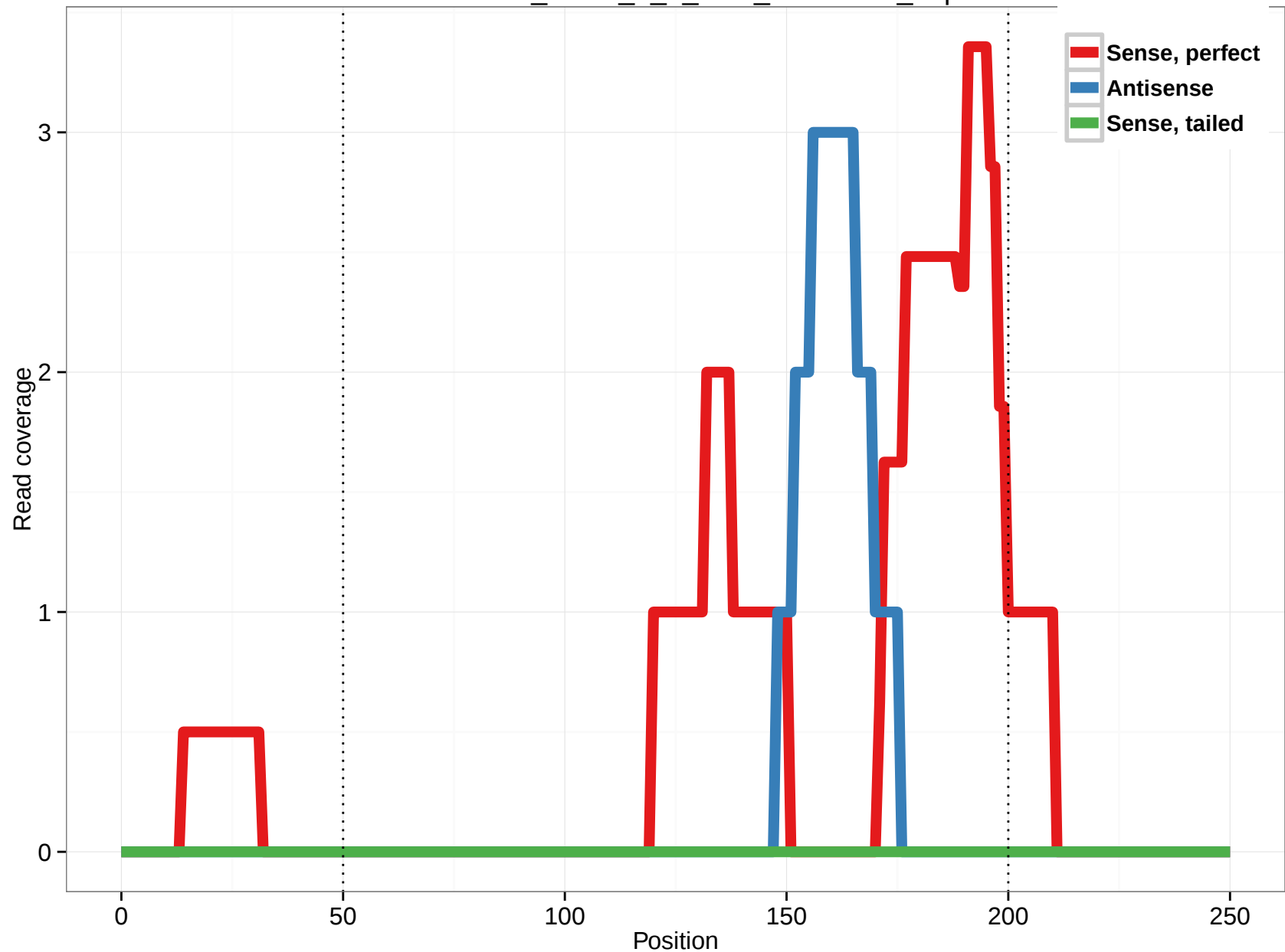
uc003tzh.1_intron_0_0_chr7_73242152_f.3p
