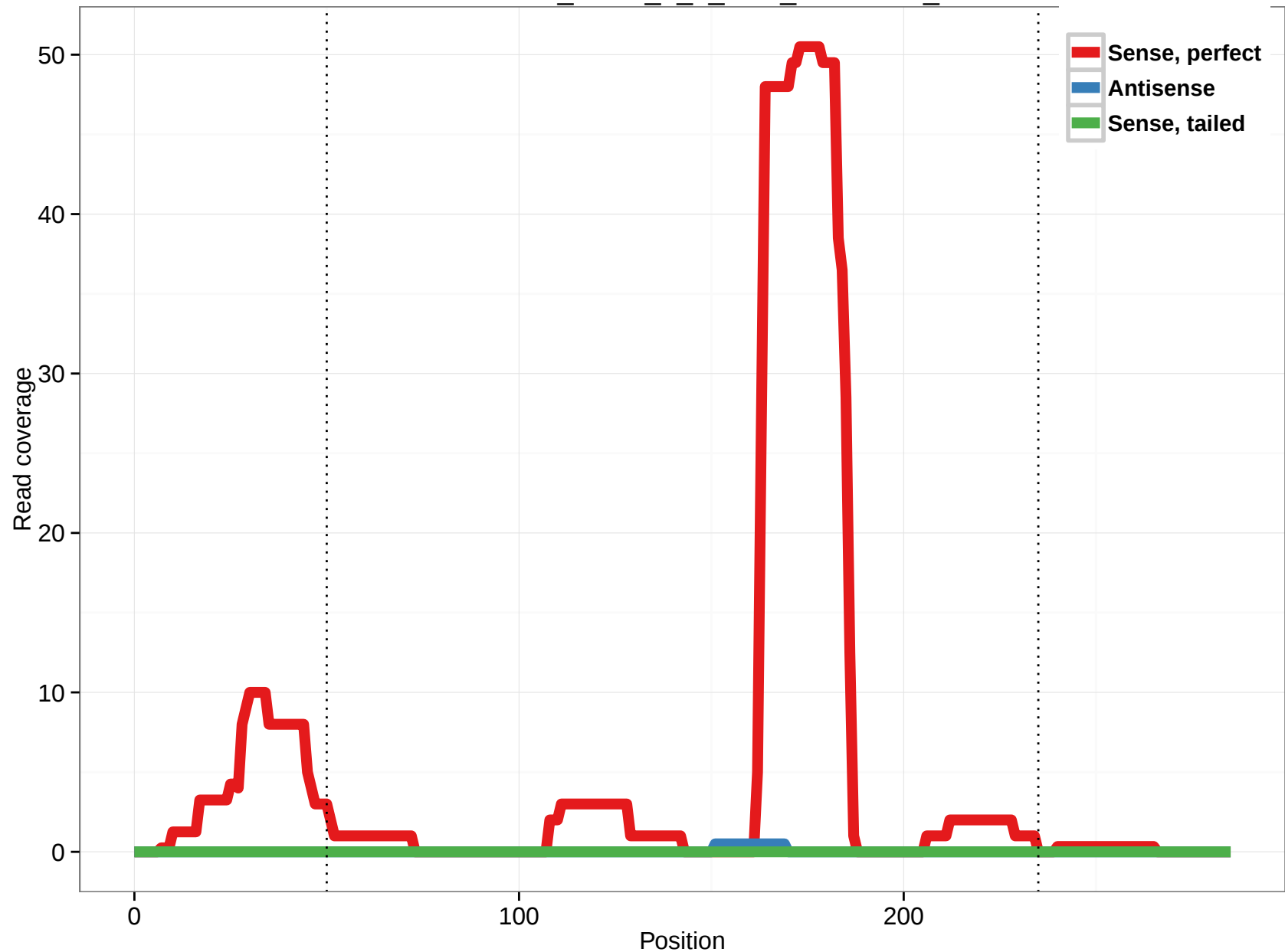
uc003tun.2_intron_8_0_chr7_65444529_r
