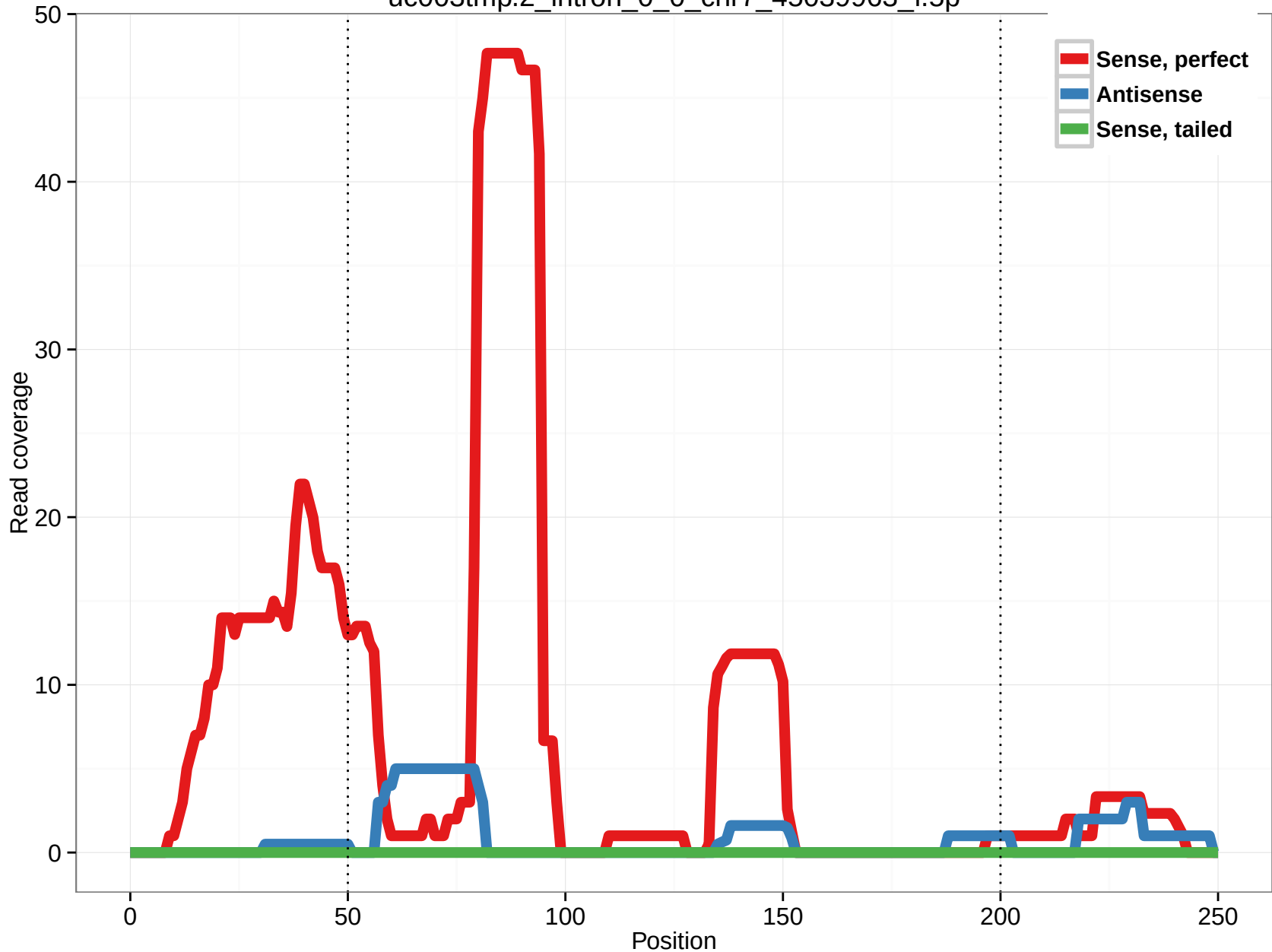
uc003tmp.2_intron_0_0_chr7_45039963_f.5p
