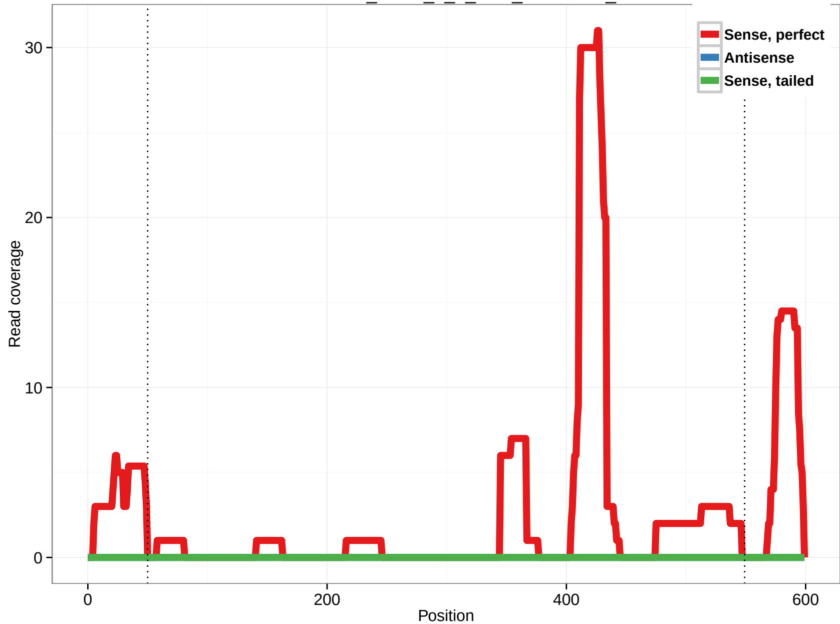
uc003tmk.3_intron_0_0_chr7_45022922_r
