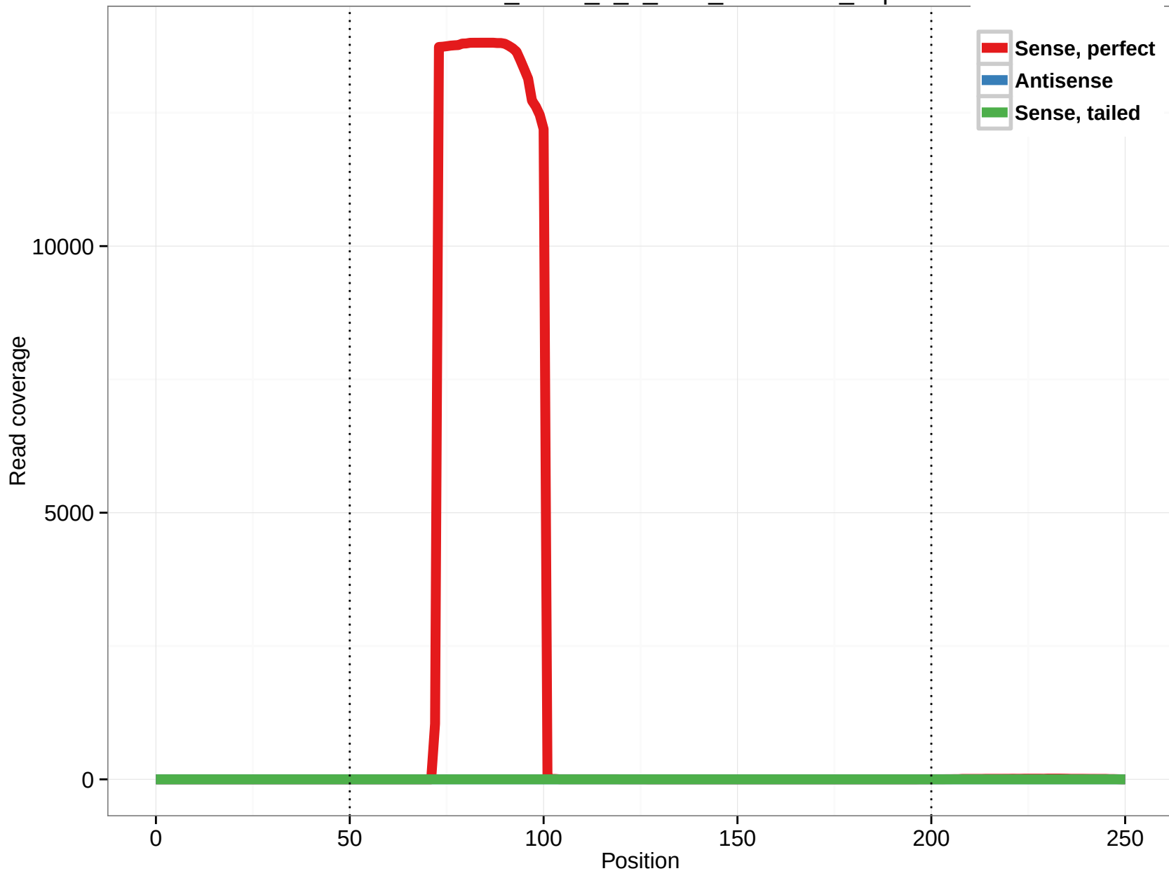
uc003tia.2_intron_1_0_chr7_42974736_f.3p
